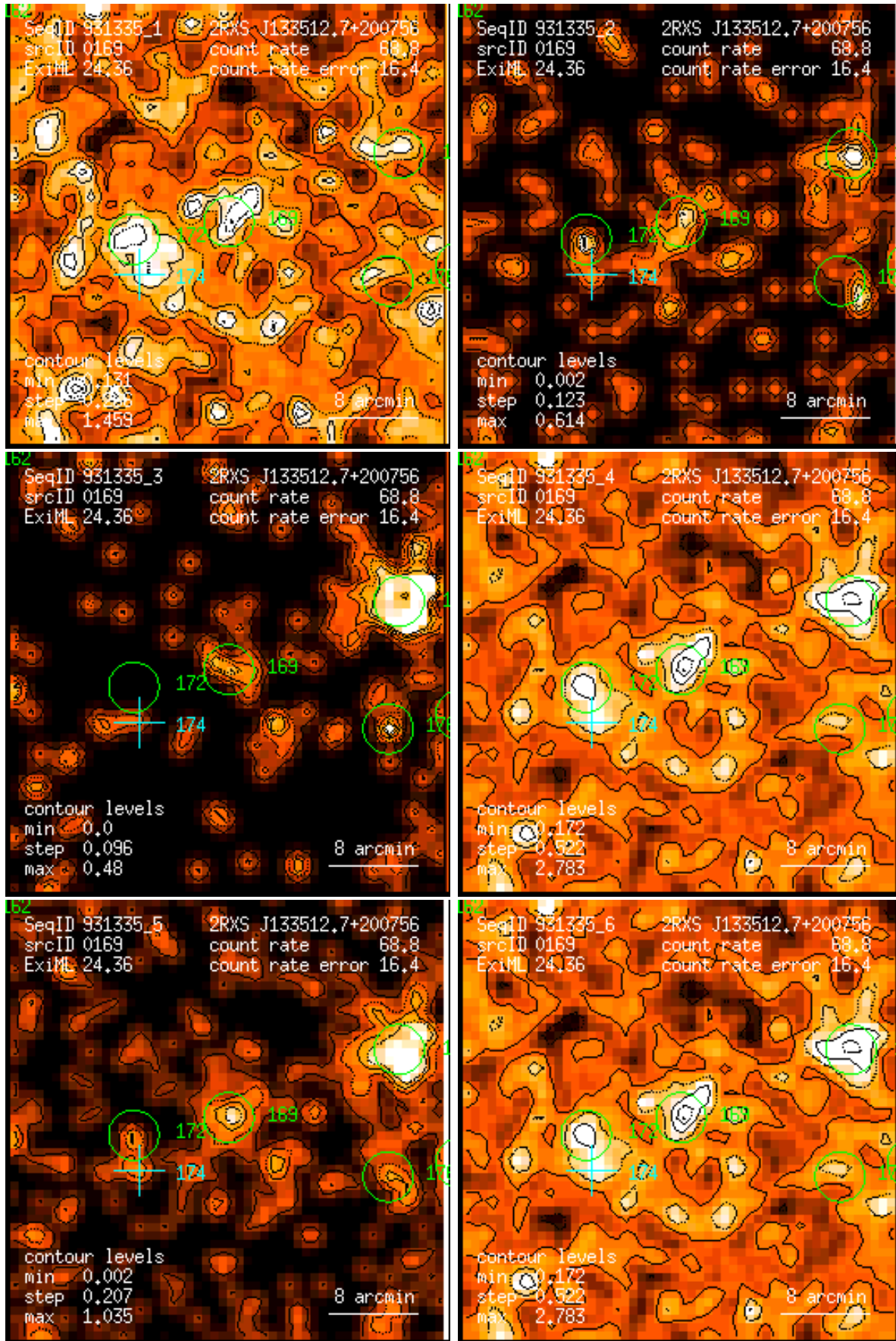
Figure 169: RASS 931335: detection 0169: band rate images, Gaussian filter: (1) PSPC channels 11 – 41, (2) 52 – 90, (3) 91 – 201, (4) 11 – 235, (5) 52 – 201, (6) 11 – 201. Broad band rates in counts/ks. Band rate contour levels in counts/ks/arcmin 2 .
