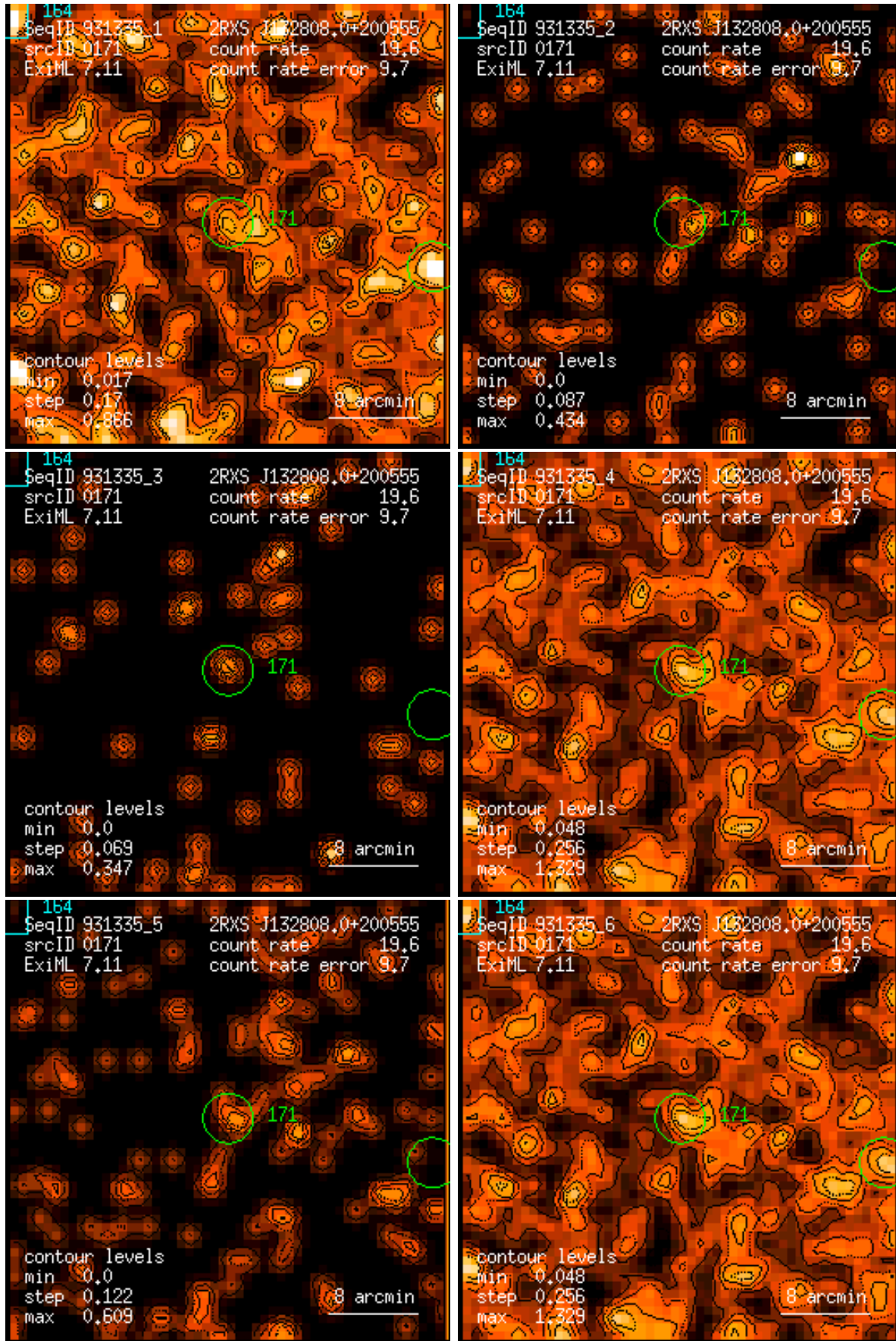
Figure 171: RASS 931335: detection 0171: band rate images, Gaussian filter: (1) PSPC channels 11 – 41, (2) 52 – 90, (3) 91 – 201, (4) 11 – 235, (5) 52 – 201, (6) 11 – 201. Broad band rates in counts/ks. Band rate contour levels in counts/ks/arcmin 2 .
