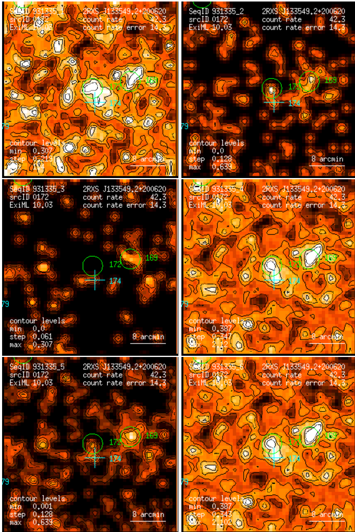
Figure 172: RASS 931335: detection 0172: band rate images, Gaussian filter: (1) PSPC channels 11 – 41, (2) 52 – 90, (3) 91 – 201, (4) 11 – 235, (5) 52 – 201, (6) 11 – 201. Broad band rates in counts/ks. Band rate contour levels in counts/ks/arcmin 2 .
