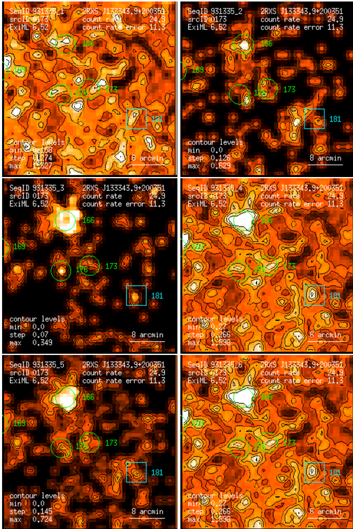
Figure 173: RASS 931335: detection 0173: band rate images, Gaussian filter: (1) PSPC channels 11 – 41, (2) 52 – 90, (3) 91 – 201, (4) 11 – 235, (5) 52 – 201, (6) 11 – 201. Broad band rates in counts/ks. Band rate contour levels in counts/ks/arcmin 2 .
