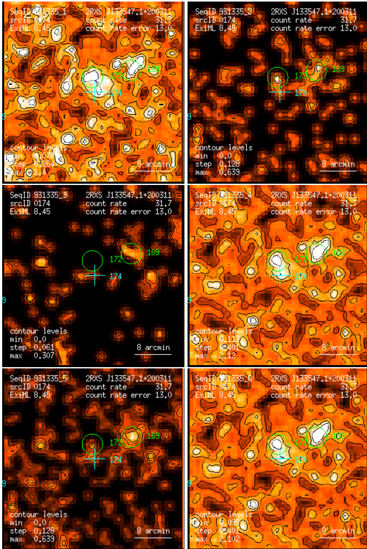
Figure 174: RASS 931335: detection 0174: band rate images, Gaussian filter: (1) PSPC channels 11 – 41, (2) 52 – 90, (3) 91 – 201, (4) 11 – 235, (5) 52 – 201, (6) 11 – 201. Broad band rates in counts/ks. Band rate contour levels in counts/ks/arcmin 2 .
