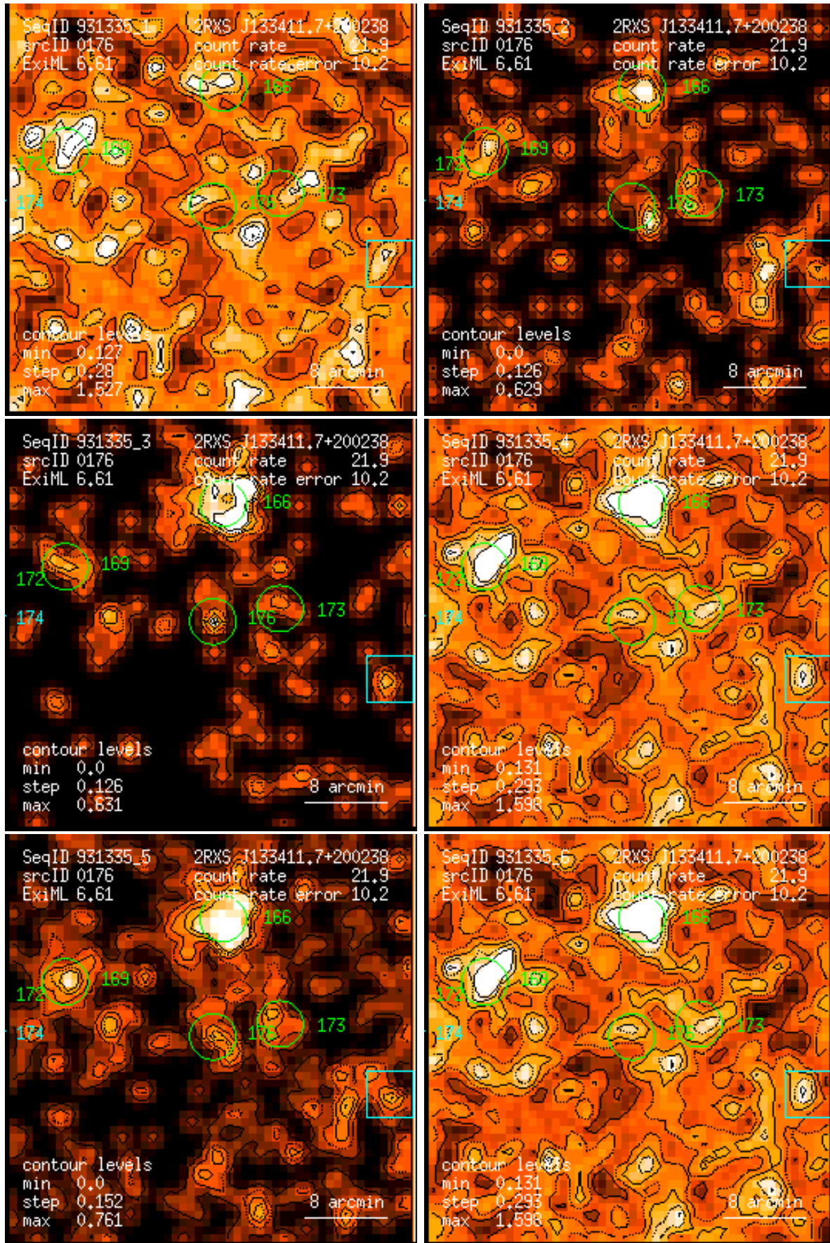
Figure 176: RASS 931335: detection 0176: band rate images, Gaussian filter: (1) PSPC channels 11 – 41, (2) 52 – 90, (3) 91 – 201, (4) 11 – 235, (5) 52 – 201, (6) 11 – 201. Broad band rates in counts/ks. Band rate contour levels in counts/ks/arcmin 2 .
