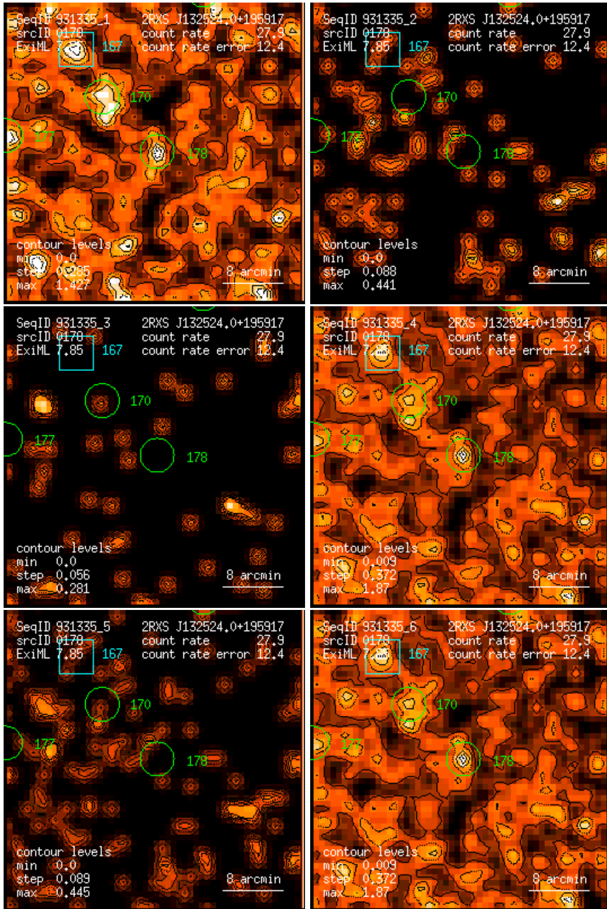
Figure 178: RASS 931335: detection 0178: band rate images, Gaussian filter: (1) PSPC channels 11 – 41, (2) 52 – 90, (3) 91 – 201, (4) 11 – 235, (5) 52 – 201, (6) 11 – 201. Broad band rates in counts/ks. Band rate contour levels in counts/ks/arcmin 2 .
