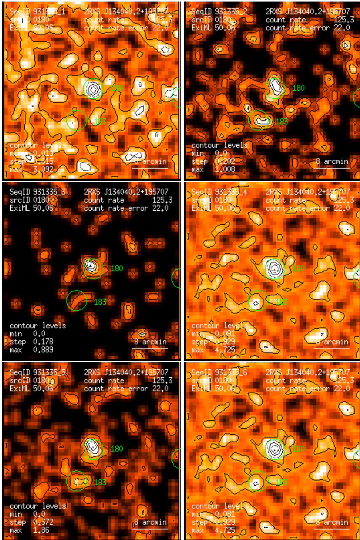
Figure 180: RASS 931335: detection 0180: band rate images, Gaussian filter: (1) PSPC channels 11 – 41, (2) 52 – 90, (3) 91 – 201, (4) 11 – 235, (5) 52 – 201, (6) 11 – 201. Broad band rates in counts/ks. Band rate contour levels in counts/ks/arcmin 2 .
