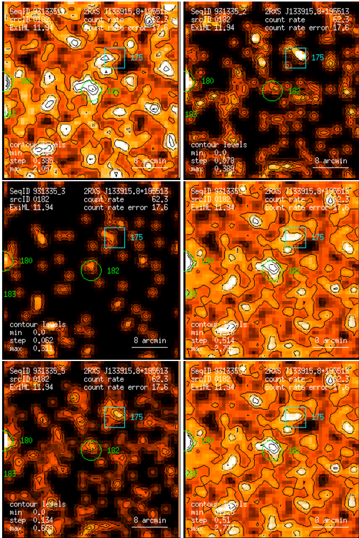
Figure 182: RASS 931335: detection 0182: band rate images, Gaussian filter: (1) PSPC channels 11 – 41, (2) 52 – 90, (3) 91 – 201, (4) 11 – 235, (5) 52 – 201, (6) 11 – 201. Broad band rates in counts/ks. Band rate contour levels in counts/ks/arcmin 2 .
