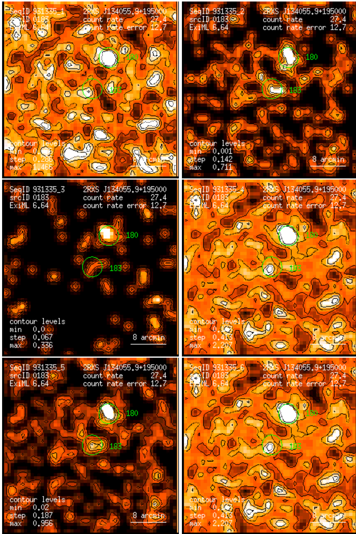
Figure 183: RASS 931335: detection 0183: band rate images, Gaussian filter: (1) PSPC channels 11 – 41, (2) 52 – 90, (3) 91 – 201, (4) 11 – 235, (5) 52 – 201, (6) 11 – 201. Broad band rates in counts/ks. Band rate contour levels in counts/ks/arcmin 2 .
