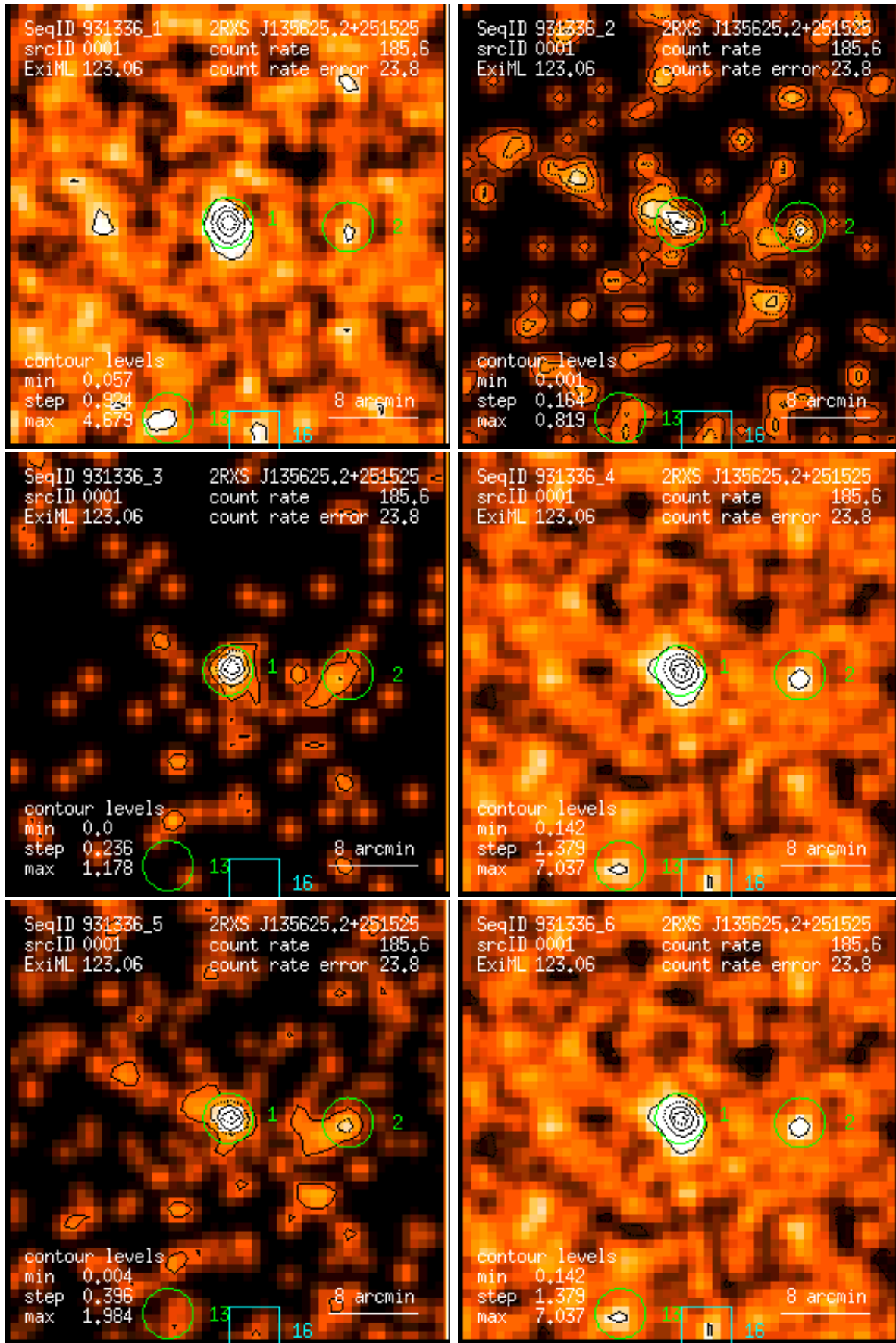
Figure 1: RASS 931336: detection 0001: band rate images, Gaussian filter: (1) PSPC channels 11 – 41, (2) 52 – 90, (3) 91 – 201, (4) 11 – 235, (5) 52 – 201, (6) 11 – 201. Broad band rates in counts/ks. Band rate contour levels in counts/ks/arcmin 2 .
