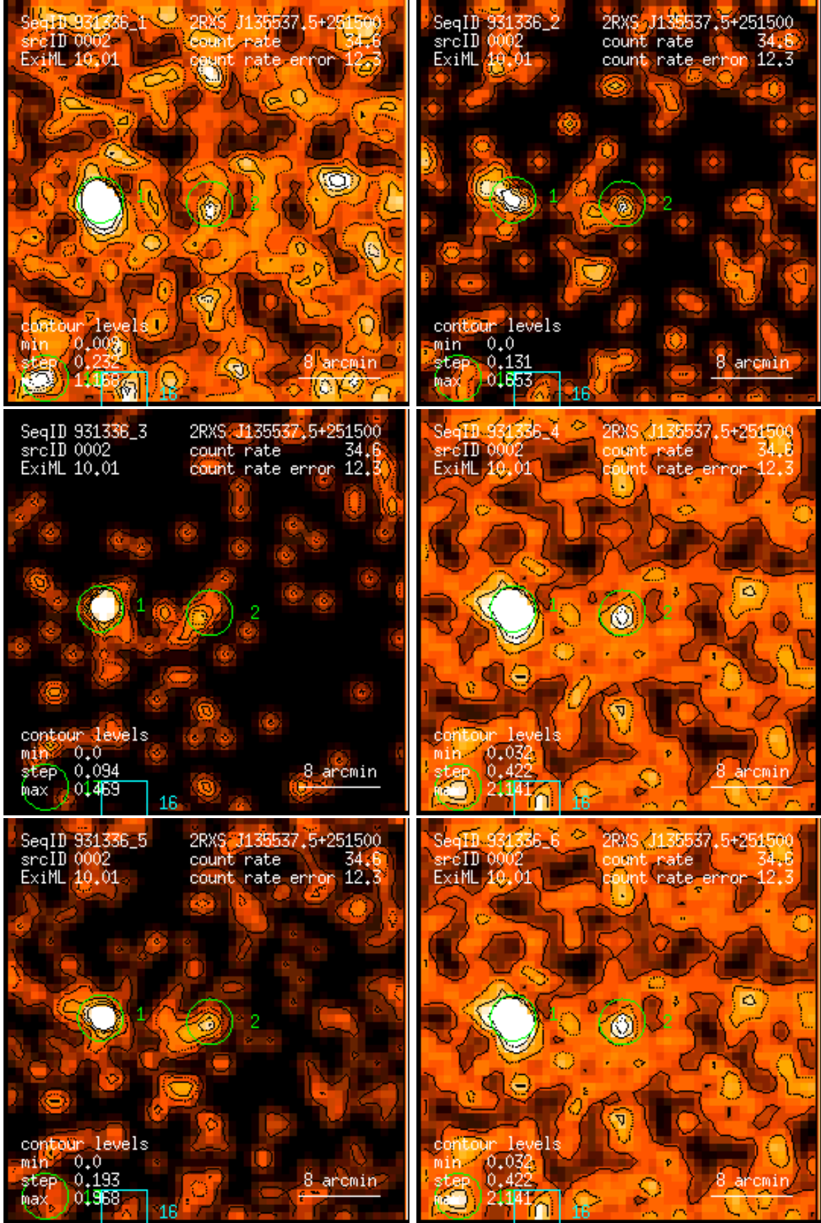
Figure 2: RASS 931336: detection 0002: band rate images, Gaussian filter: (1) PSPC channels 11 – 41, (2) 52 – 90, (3) 91 – 201, (4) 11 – 235, (5) 52 – 201, (6) 11 – 201. Broad band rates in counts/ks. Band rate contour levels in counts/ks/arcmin 2 .
