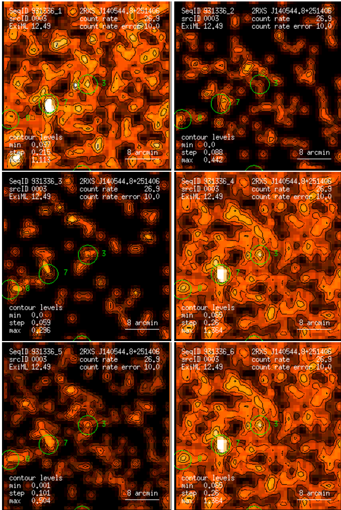
Figure 3: RASS 931336: detection 0003: band rate images, Gaussian filter: (1) PSPC channels 11 – 41, (2) 52 – 90, (3) 91 – 201, (4) 11 – 235, (5) 52 – 201, (6) 11 – 201. Broad band rates in counts/ks. Band rate contour levels in counts/ks/arcmin 2 .
