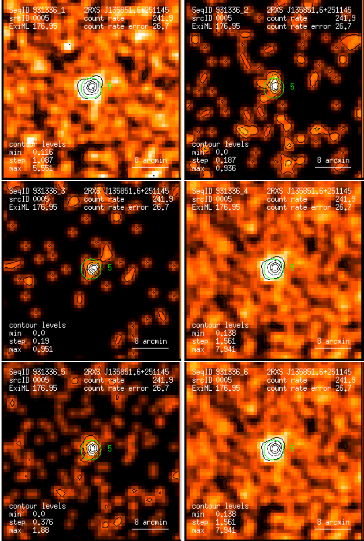
Figure 5: RASS 931336: detection 0005: band rate images, Gaussian filter: (1) PSPC channels 11 – 41, (2) 52 – 90, (3) 91 – 201, (4) 11 – 235, (5) 52 – 201, (6) 11 – 201. Broad band rates in counts/ks. Band rate contour levels in counts/ks/arcmin 2 .
