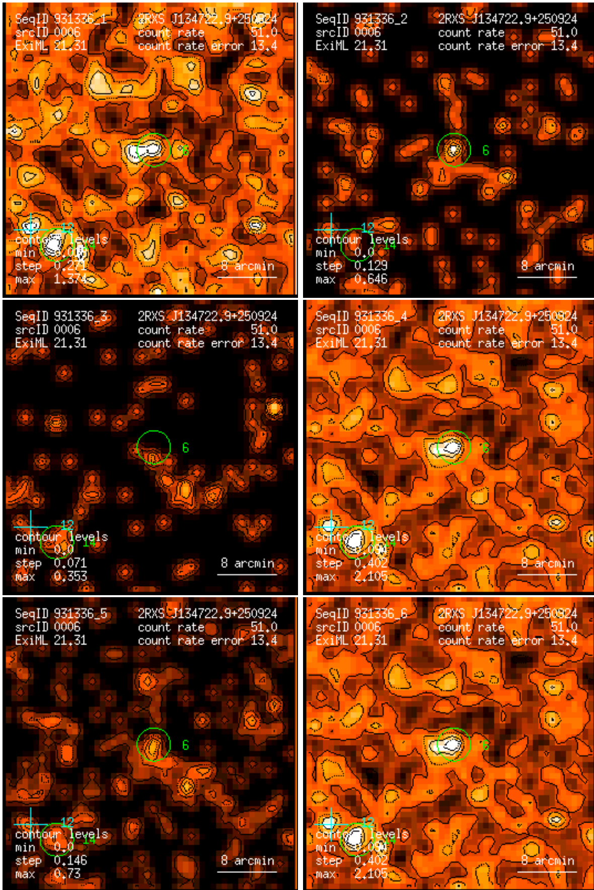
Figure 6: RASS 931336: detection 0006: band rate images, Gaussian filter: (1) PSPC channels 11 – 41, (2) 52 – 90, (3) 91 – 201, (4) 11 – 235, (5) 52 – 201, (6) 11 – 201. Broad band rates in counts/ks. Band rate contour levels in counts/ks/arcmin 2 .
