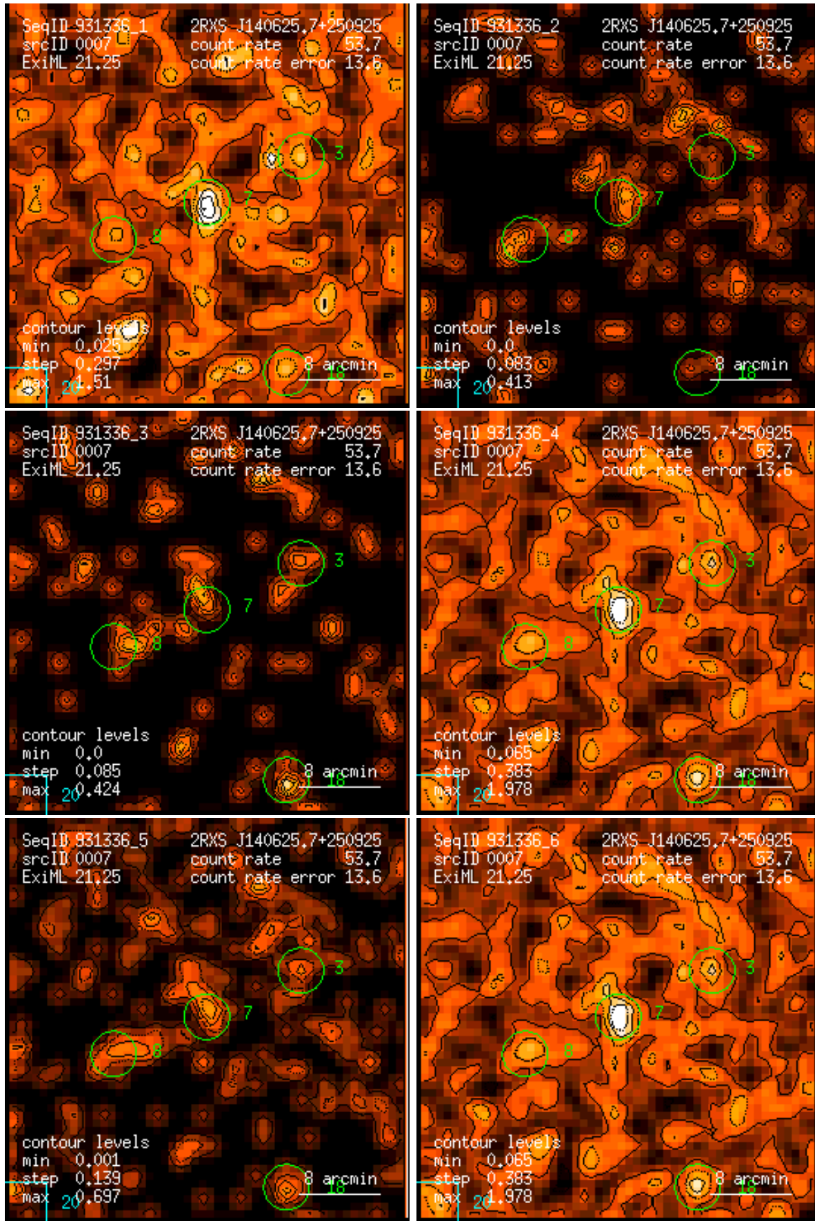
Figure 7: RASS 931336: detection 0007: band rate images, Gaussian filter: (1) PSPC channels 11 – 41, (2) 52 – 90, (3) 91 – 201, (4) 11 – 235, (5) 52 – 201, (6) 11 – 201. Broad band rates in counts/ks. Band rate contour levels in counts/ks/arcmin 2 .
