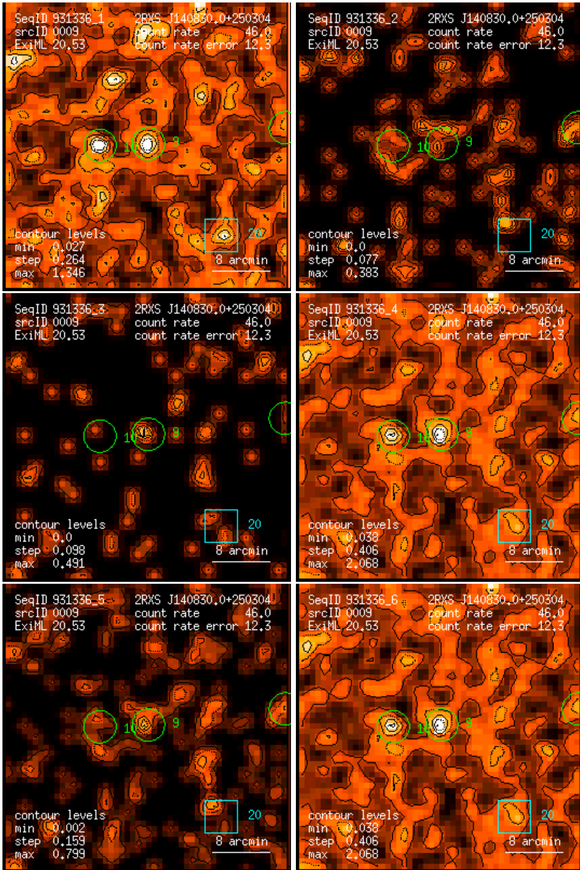
Figure 9: RASS 931336: detection 0009: band rate images, Gaussian filter: (1) PSPC channels 11 – 41, (2) 52 – 90, (3) 91 – 201, (4) 11 – 235, (5) 52 – 201, (6) 11 – 201. Broad band rates in counts/ks. Band rate contour levels in counts/ks/arcmin 2 .
