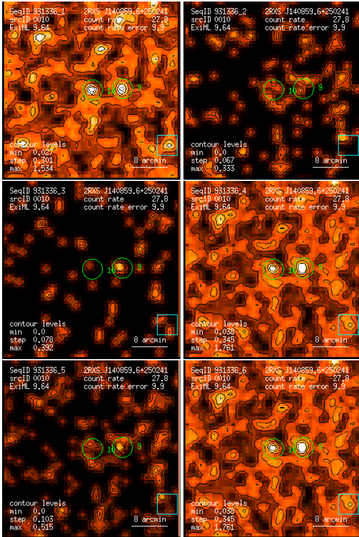
Figure 10: RASS 931336: detection 0010: band rate images, Gaussian filter: (1) PSPC channels 11 – 41, (2) 52 – 90, (3) 91 – 201, (4) 11 – 235, (5) 52 – 201, (6) 11 – 201. Broad band rates in counts/ks. Band rate contour levels in counts/ks/arcmin 2 .
