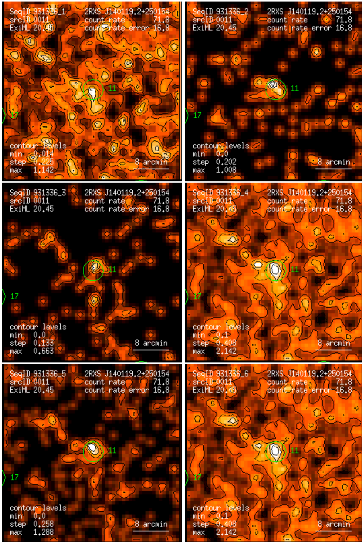
Figure 11: RASS 931336: detection 0011: band rate images, Gaussian filter: (1) PSPC channels 11 – 41, (2) 52 – 90, (3) 91 – 201, (4) 11 – 235, (5) 52 – 201, (6) 11 – 201. Broad band rates in counts/ks. Band rate contour levels in counts/ks/arcmin 2 .
