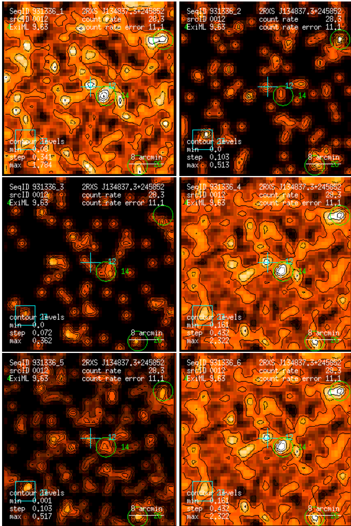
Figure 12: RASS 931336: detection 0012: band rate images, Gaussian filter: (1) PSPC channels 11 – 41, (2) 52 – 90, (3) 91 – 201, (4) 11 – 235, (5) 52 – 201, (6) 11 – 201. Broad band rates in counts/ks. Band rate contour levels in counts/ks/arcmin 2 .
