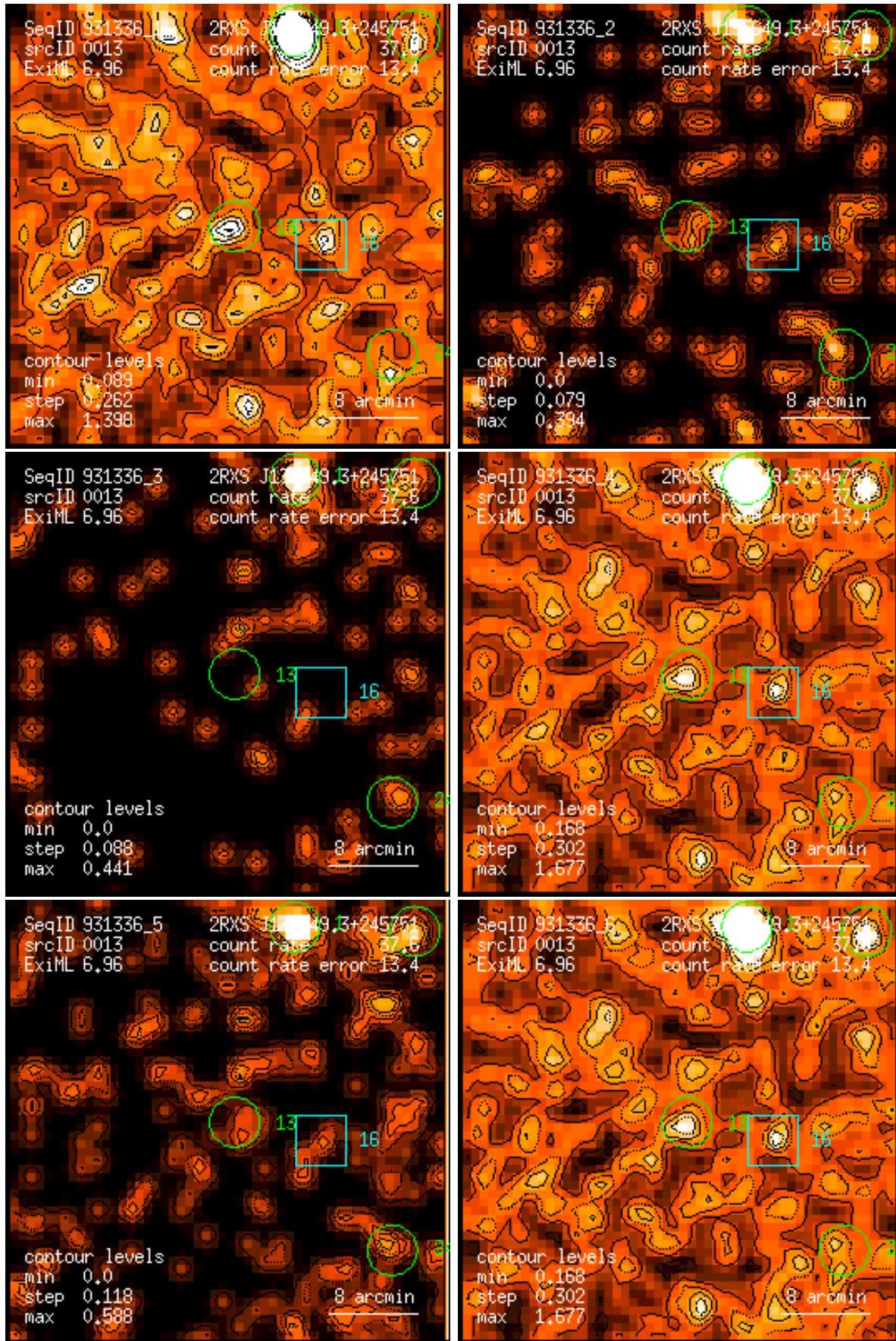
Figure 13: RASS 931336: detection 0013: band rate images, Gaussian filter: (1) PSPC channels 11 – 41, (2) 52 – 90, (3) 91 – 201, (4) 11 – 235, (5) 52 – 201, (6) 11 – 201. Broad band rates in counts/ks. Band rate contour levels in counts/ks/arcmin 2 .
