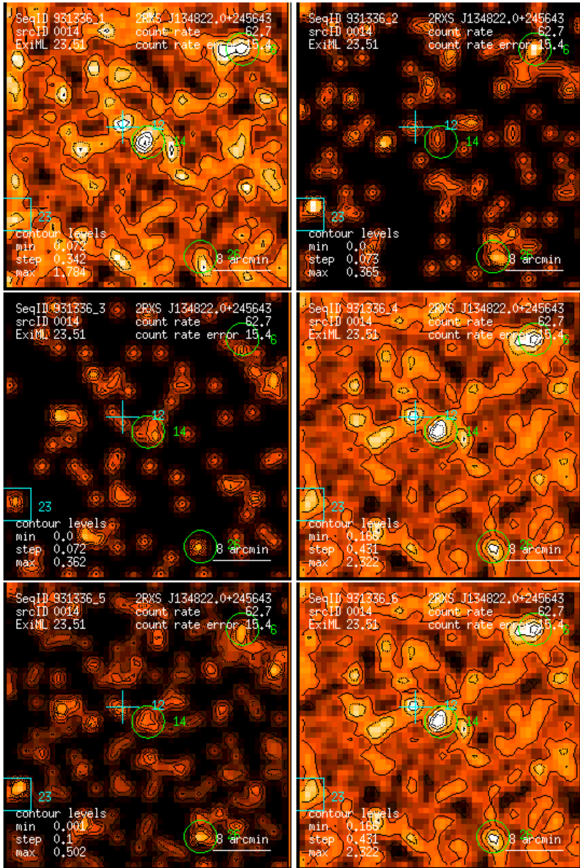
Figure 14: RASS 931336: detection 0014: band rate images, Gaussian filter: (1) PSPC channels 11 – 41, (2) 52 – 90, (3) 91 – 201, (4) 11 – 235, (5) 52 – 201, (6) 11 – 201. Broad band rates in counts/ks. Band rate contour levels in counts/ks/arcmin 2 .
