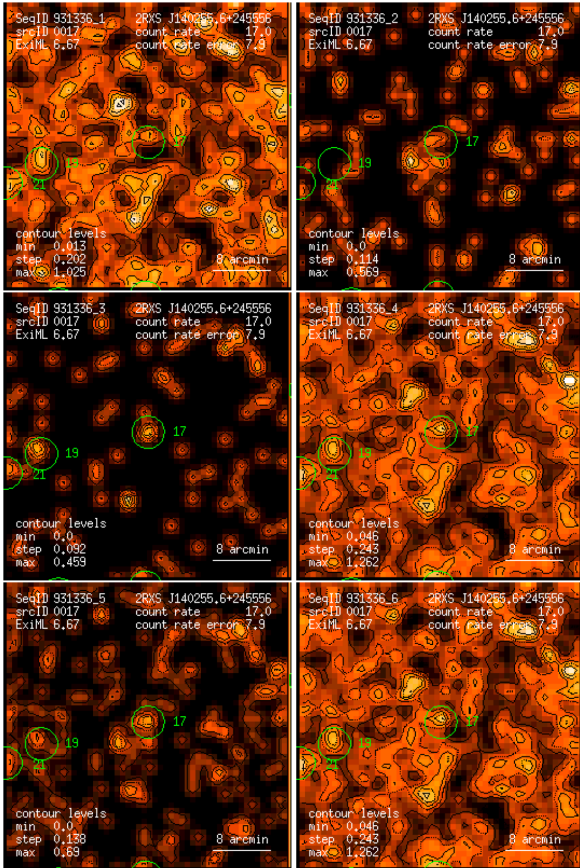
Figure 17: RASS 931336: detection 0017: band rate images, Gaussian filter: (1) PSPC channels 11 – 41, (2) 52 – 90, (3) 91 – 201, (4) 11 – 235, (5) 52 – 201, (6) 11 – 201. Broad band rates in counts/ks. Band rate contour levels in counts/ks/arcmin 2 .
