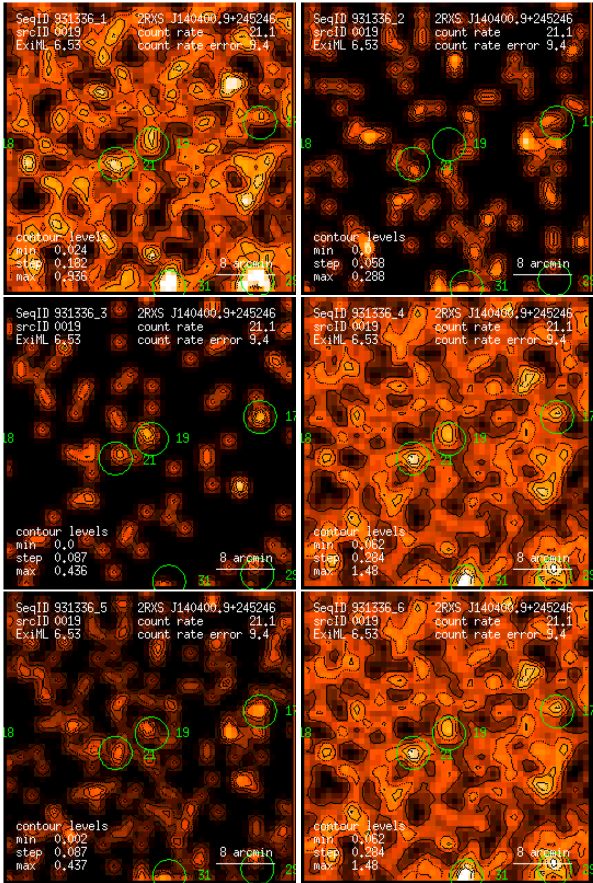
Figure 19: RASS 931336: detection 0019: band rate images, Gaussian filter: (1) PSPC channels 11 – 41, (2) 52 – 90, (3) 91 – 201, (4) 11 – 235, (5) 52 – 201, (6) 11 – 201. Broad band rates in counts/ks. Band rate contour levels in counts/ks/arcmin 2 .
