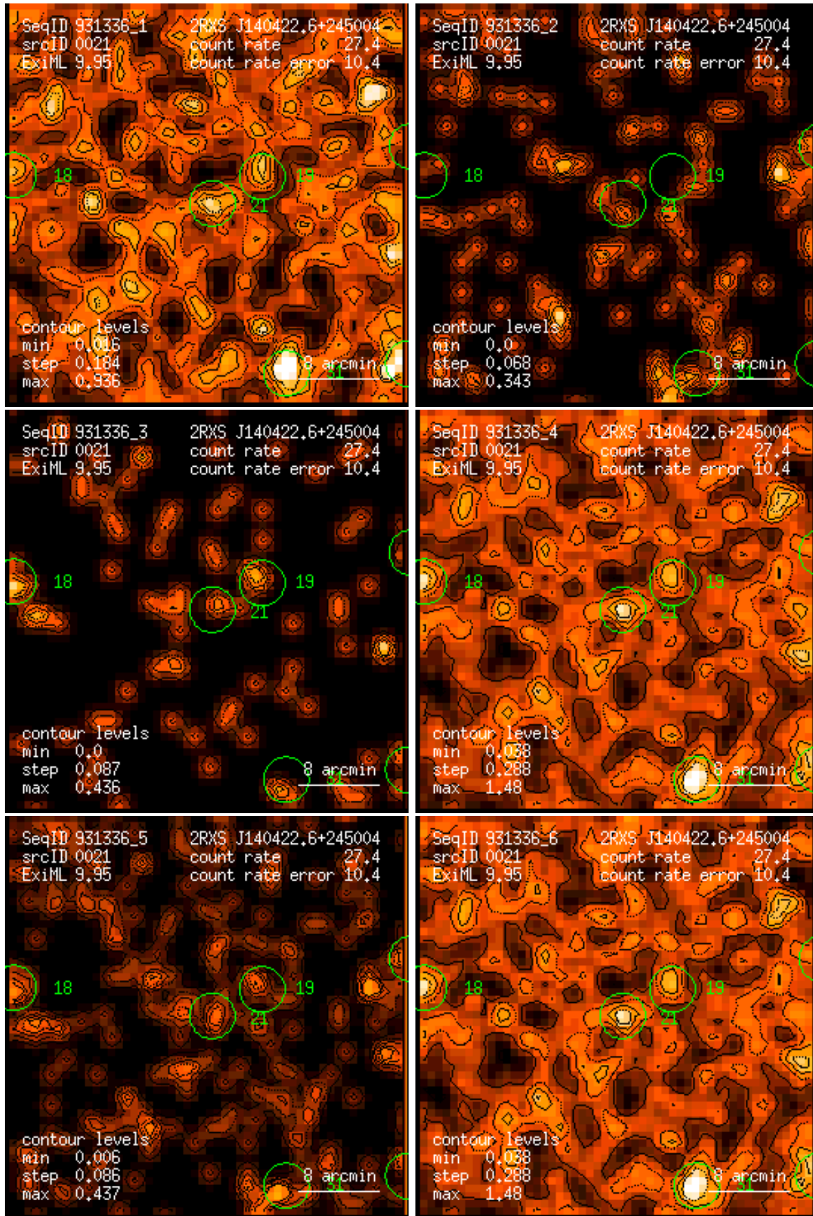
Figure 21: RASS 931336: detection 0021: band rate images, Gaussian filter: (1) PSPC channels 11 – 41, (2) 52 – 90, (3) 91 – 201, (4) 11 – 235, (5) 52 – 201, (6) 11 – 201. Broad band rates in counts/ks. Band rate contour levels in counts/ks/arcmin 2 .
