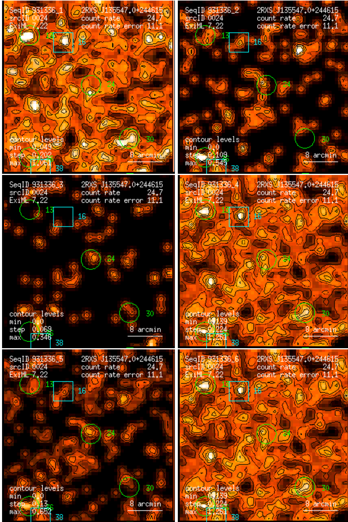
Figure 24: RASS 931336: detection 0024: band rate images, Gaussian filter: (1) PSPC channels 11 – 41, (2) 52 – 90, (3) 91 – 201, (4) 11 – 235, (5) 52 – 201, (6) 11 – 201. Broad band rates in counts/ks. Band rate contour levels in counts/ks/arcmin 2 .
