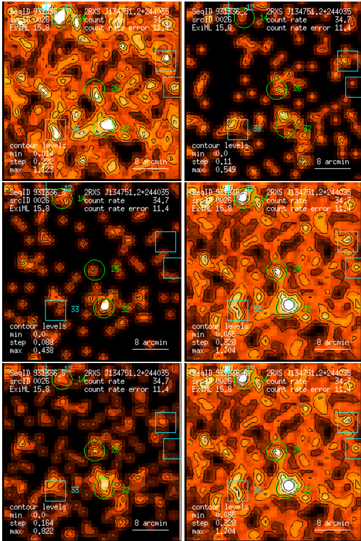
Figure 26: RASS 931336: detection 0026: band rate images, Gaussian filter: (1) PSPC channels 11 – 41, (2) 52 – 90, (3) 91 – 201, (4) 11 – 235, (5) 52 – 201, (6) 11 – 201. Broad band rates in counts/ks. Band rate contour levels in counts/ks/arcmin 2 .
