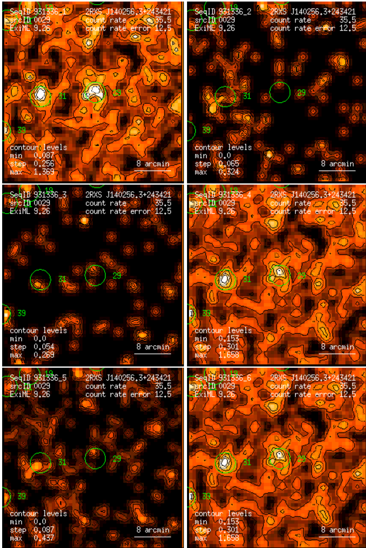
Figure 29: RASS 931336: detection 0029: band rate images, Gaussian filter: (1) PSPC channels 11 – 41, (2) 52 – 90, (3) 91 – 201, (4) 11 – 235, (5) 52 – 201, (6) 11 – 201. Broad band rates in counts/ks. Band rate contour levels in counts/ks/arcmin 2 .
