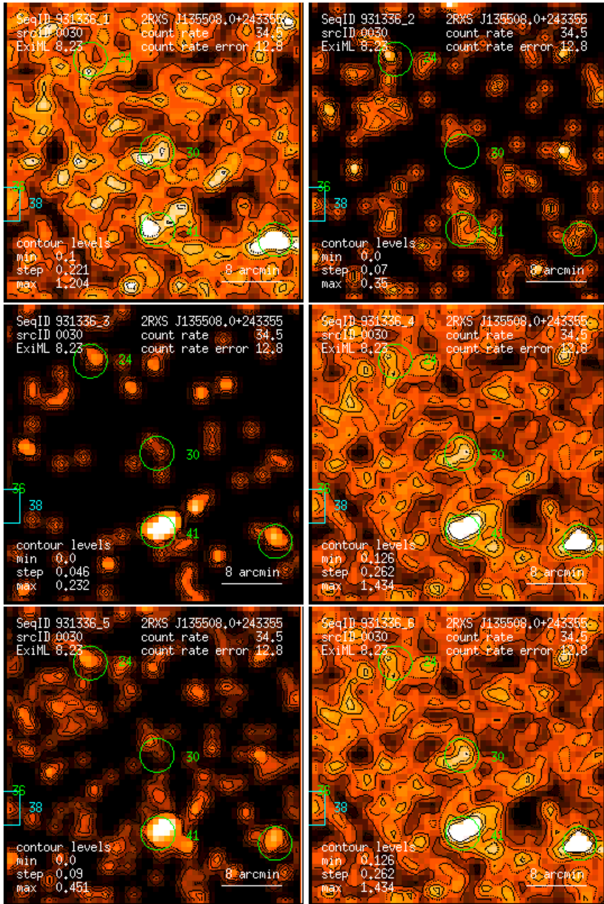
Figure 30: RASS 931336: detection 0030: band rate images, Gaussian filter: (1) PSPC channels 11 – 41, (2) 52 – 90, (3) 91 – 201, (4) 11 – 235, (5) 52 – 201, (6) 11 – 201. Broad band rates in counts/ks. Band rate contour levels in counts/ks/arcmin 2 .
