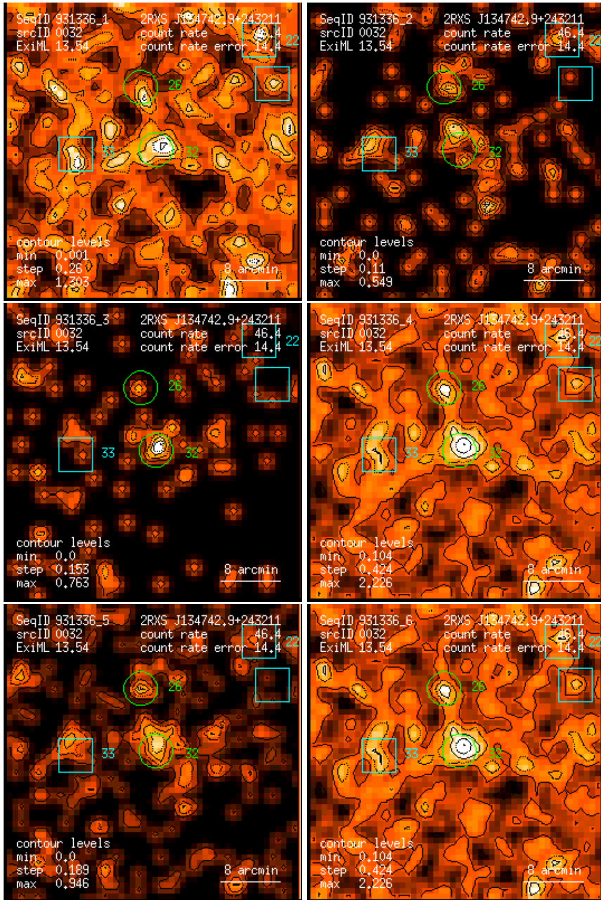
Figure 32: RASS 931336: detection 0032: band rate images, Gaussian filter: (1) PSPC channels 11 – 41, (2) 52 – 90, (3) 91 – 201, (4) 11 – 235, (5) 52 – 201, (6) 11 – 201. Broad band rates in counts/ks. Band rate contour levels in counts/ks/arcmin 2 .
