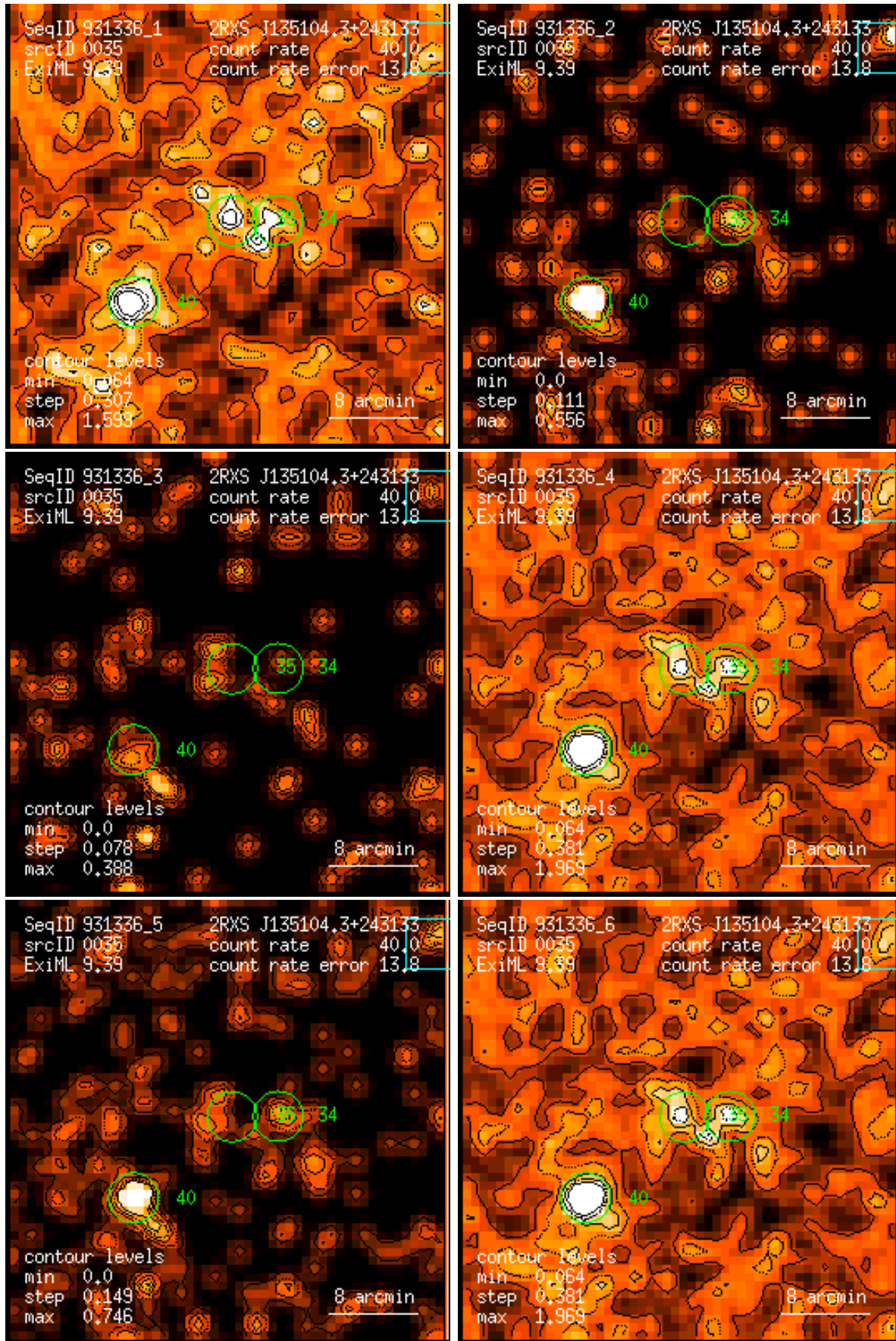
Figure 35: RASS 931336: detection 0035: band rate images, Gaussian filter: (1) PSPC channels 11 – 41, (2) 52 – 90, (3) 91 – 201, (4) 11 – 235, (5) 52 – 201, (6) 11 – 201. Broad band rates in counts/ks. Band rate contour levels in counts/ks/arcmin 2 .
