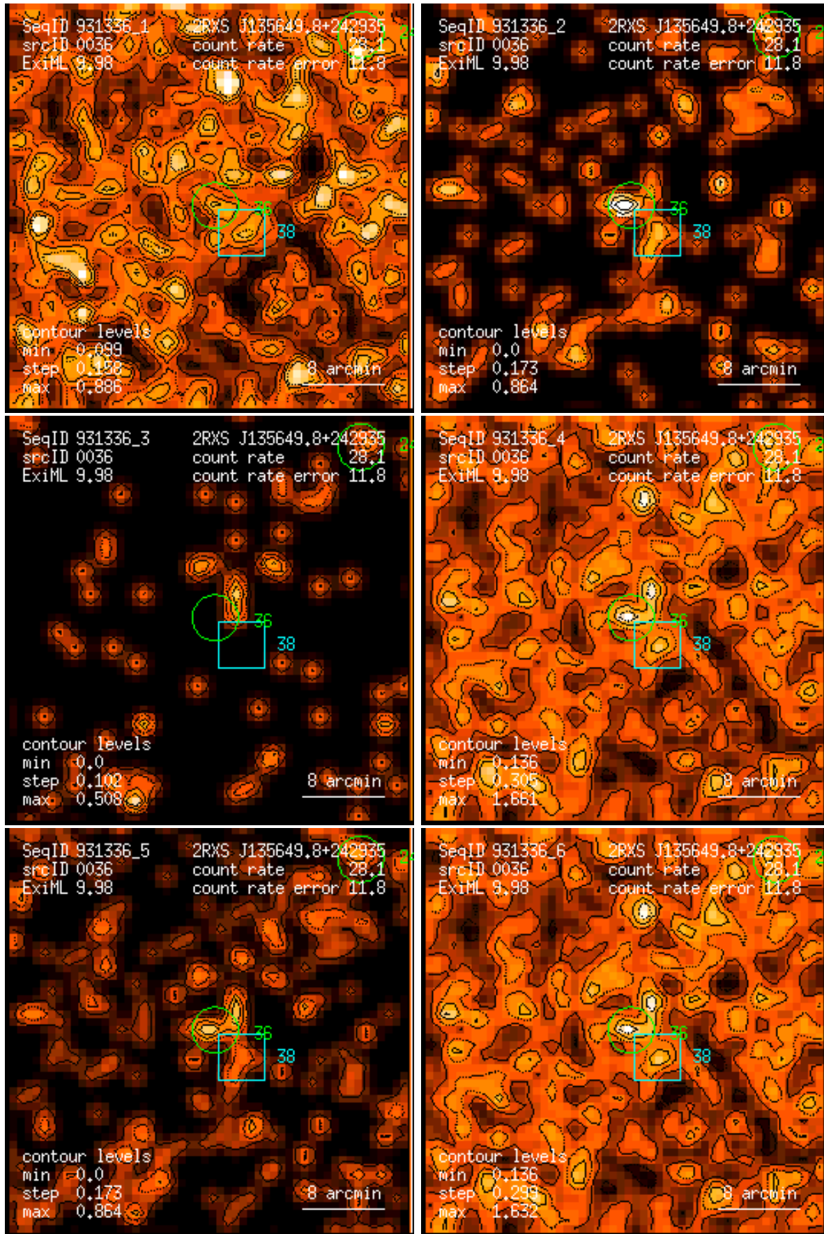
Figure 36: RASS 931336: detection 0036: band rate images, Gaussian filter: (1) PSPC channels 11 – 41, (2) 52 – 90, (3) 91 – 201, (4) 11 – 235, (5) 52 – 201, (6) 11 – 201. Broad band rates in counts/ks. Band rate contour levels in counts/ks/arcmin 2 .
