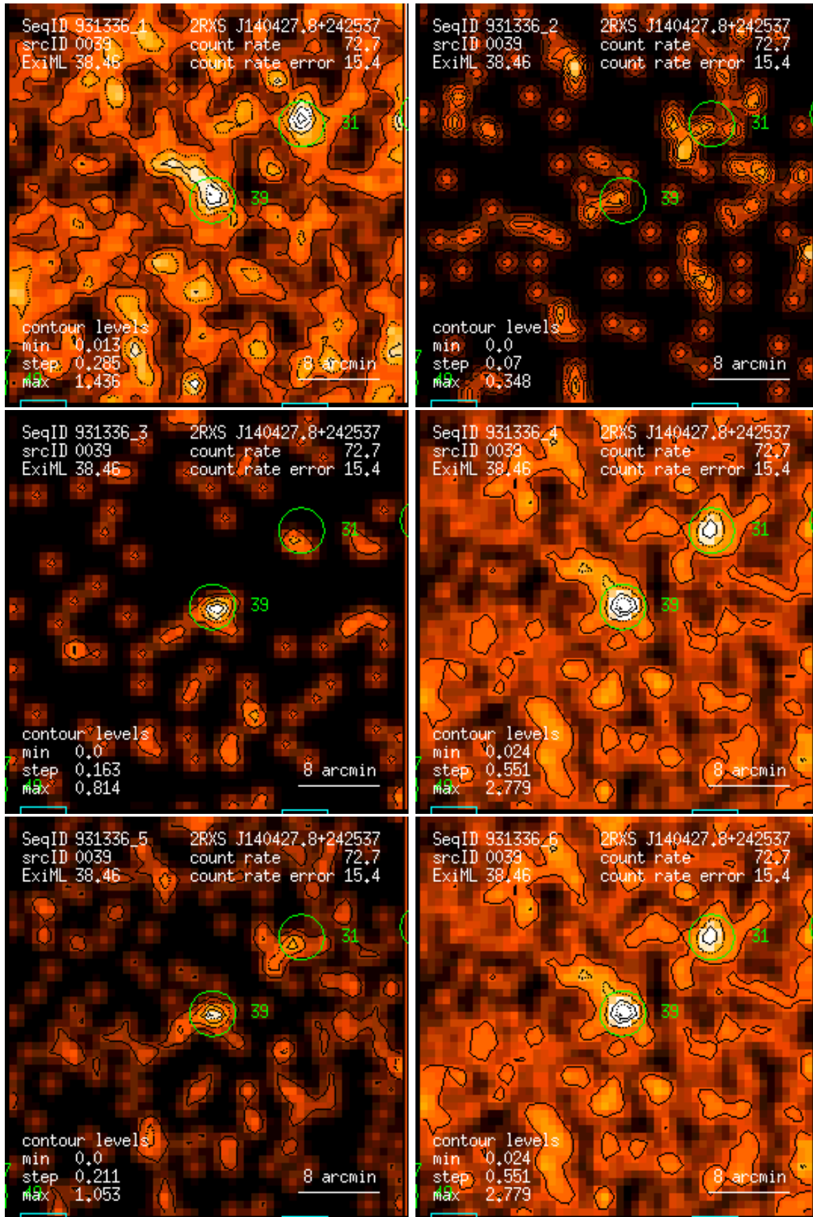
Figure 39: RASS 931336: detection 0039: band rate images, Gaussian filter: (1) PSPC channels 11 – 41, (2) 52 – 90, (3) 91 – 201, (4) 11 – 235, (5) 52 – 201, (6) 11 – 201. Broad band rates in counts/ks. Band rate contour levels in counts/ks/arcmin 2 .
