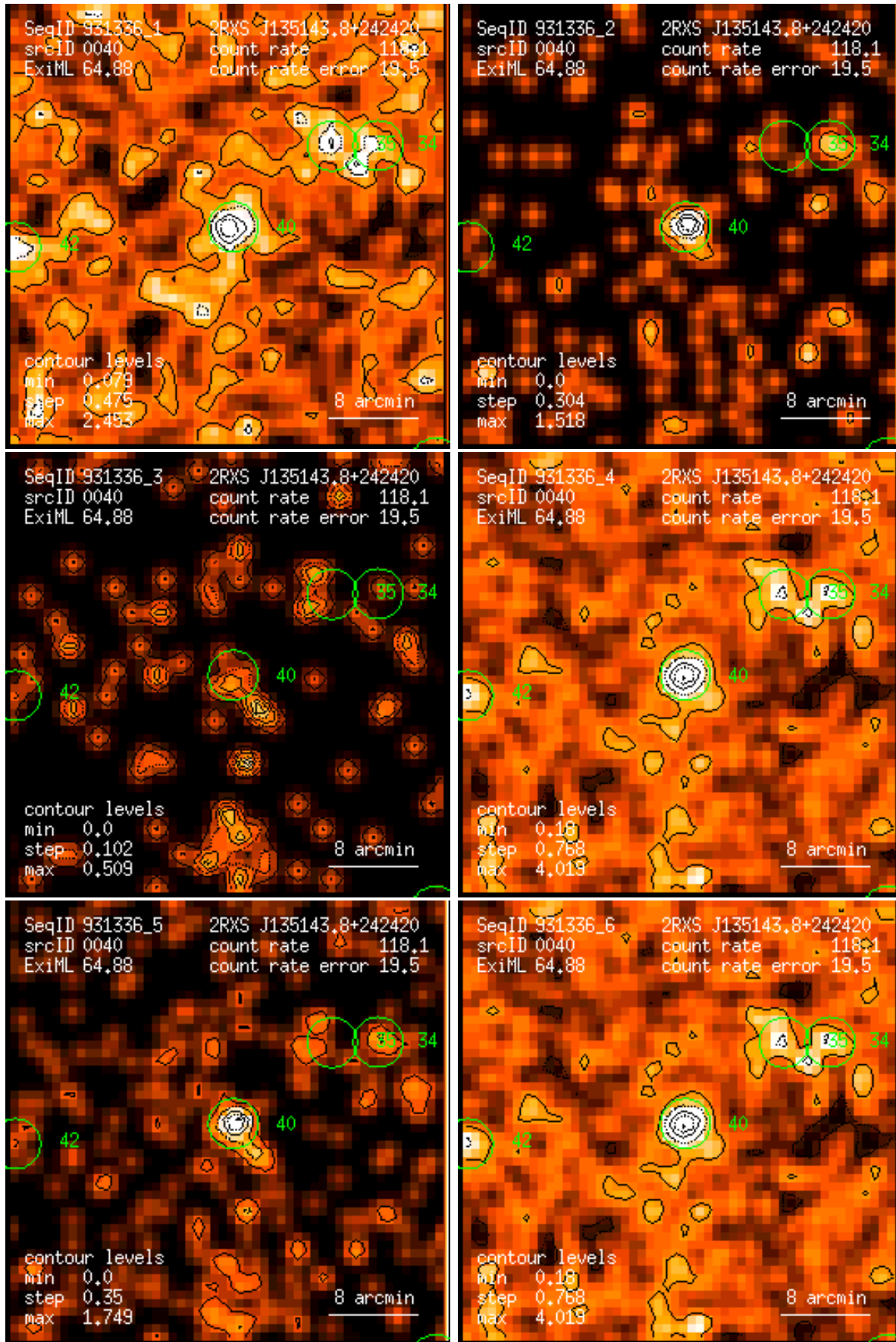
Figure 40: RASS 931336: detection 0040: band rate images, Gaussian filter: (1) PSPC channels 11 – 41, (2) 52 – 90, (3) 91 – 201, (4) 11 – 235, (5) 52 – 201, (6) 11 – 201. Broad band rates in counts/ks. Band rate contour levels in counts/ks/arcmin 2 .
