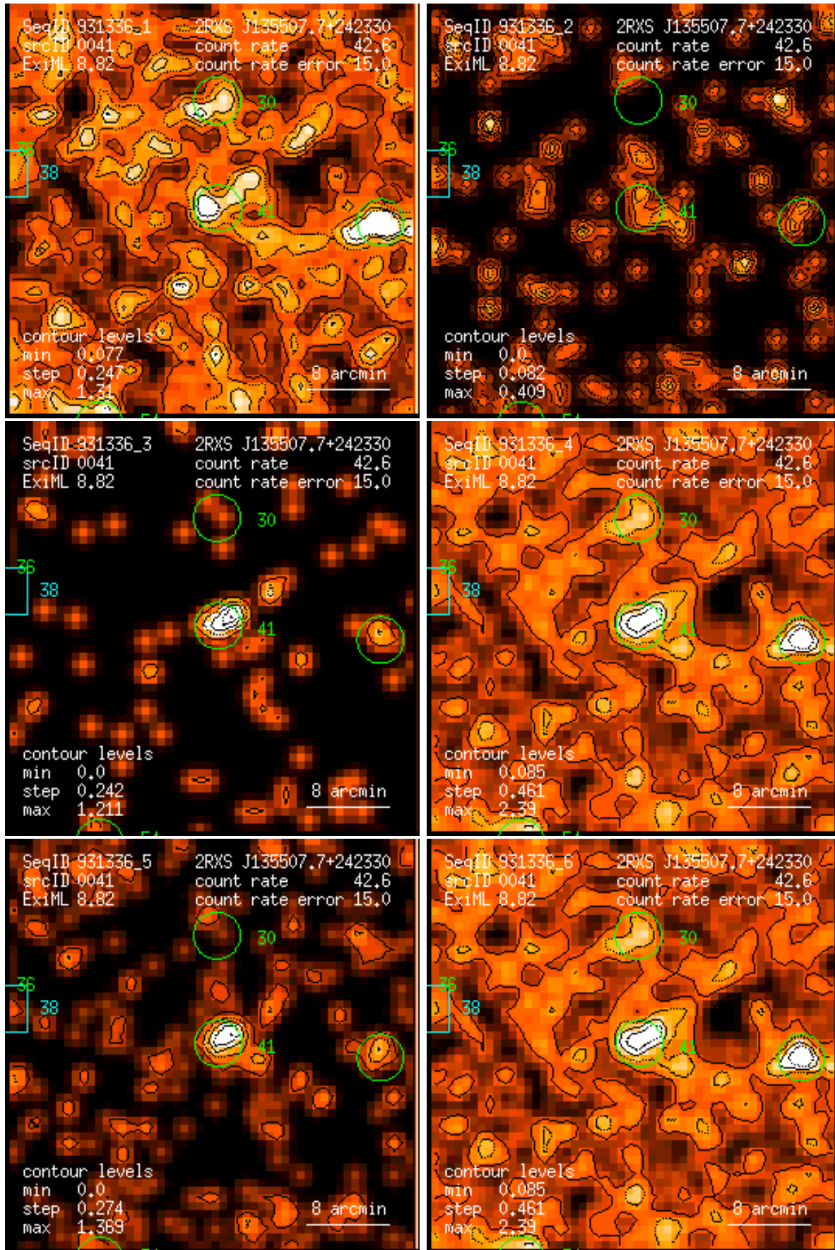
Figure 41: RASS 931336: detection 0041: band rate images, Gaussian filter: (1) PSPC channels 11 – 41, (2) 52 – 90, (3) 91 – 201, (4) 11 – 235, (5) 52 – 201, (6) 11 – 201. Broad band rates in counts/ks. Band rate contour levels in counts/ks/arcmin 2 .
