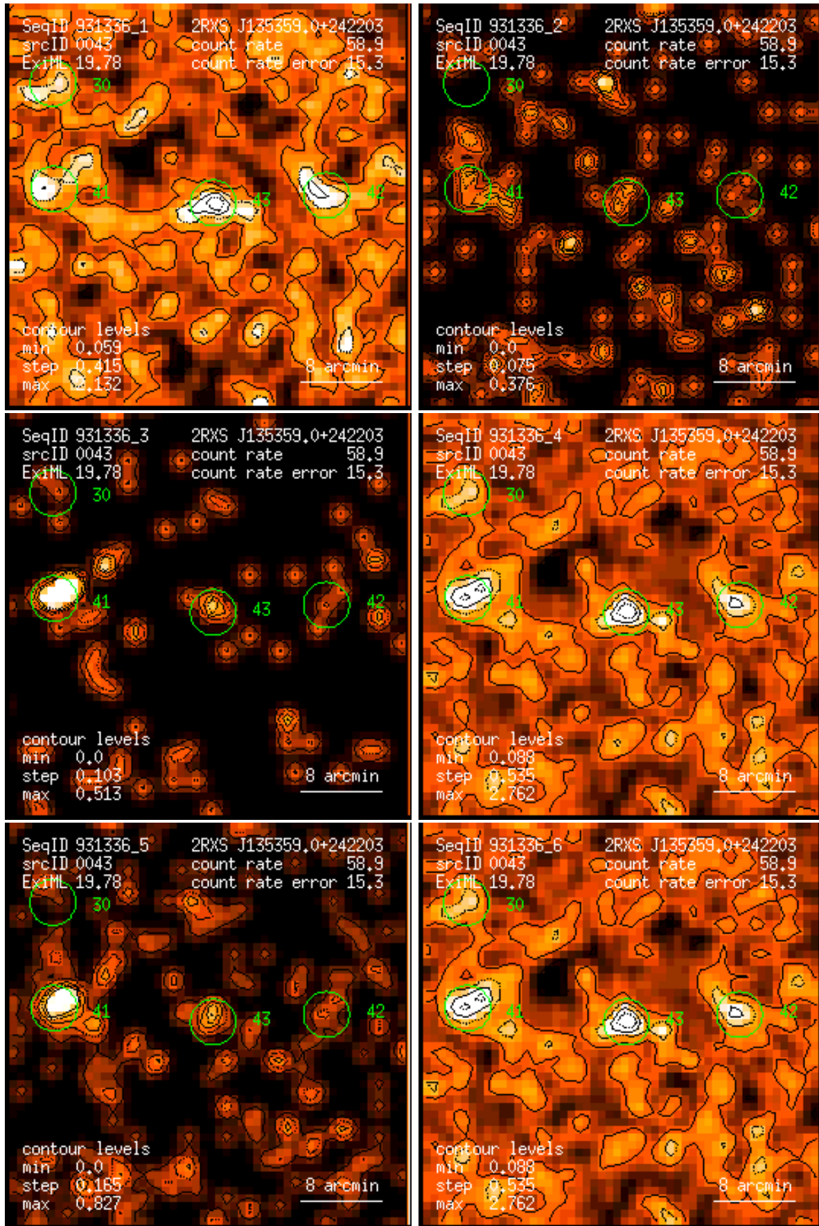
Figure 43: RASS 931336: detection 0043: band rate images, Gaussian filter: (1) PSPC channels 11 – 41, (2) 52 – 90, (3) 91 – 201, (4) 11 – 235, (5) 52 – 201, (6) 11 – 201. Broad band rates in counts/ks. Band rate contour levels in counts/ks/arcmin 2 .
