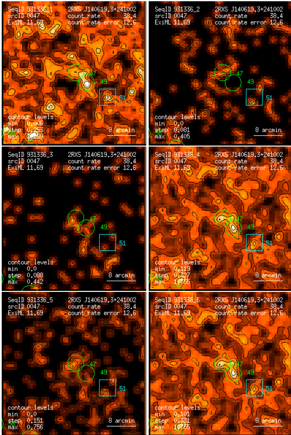
Figure 47: RASS 931336: detection 0047: band rate images, Gaussian filter: (1) PSPC channels 11 – 41, (2) 52 – 90, (3) 91 – 201, (4) 11 – 235, (5) 52 – 201, (6) 11 – 201. Broad band rates in counts/ks. Band rate contour levels in counts/ks/arcmin 2 .
