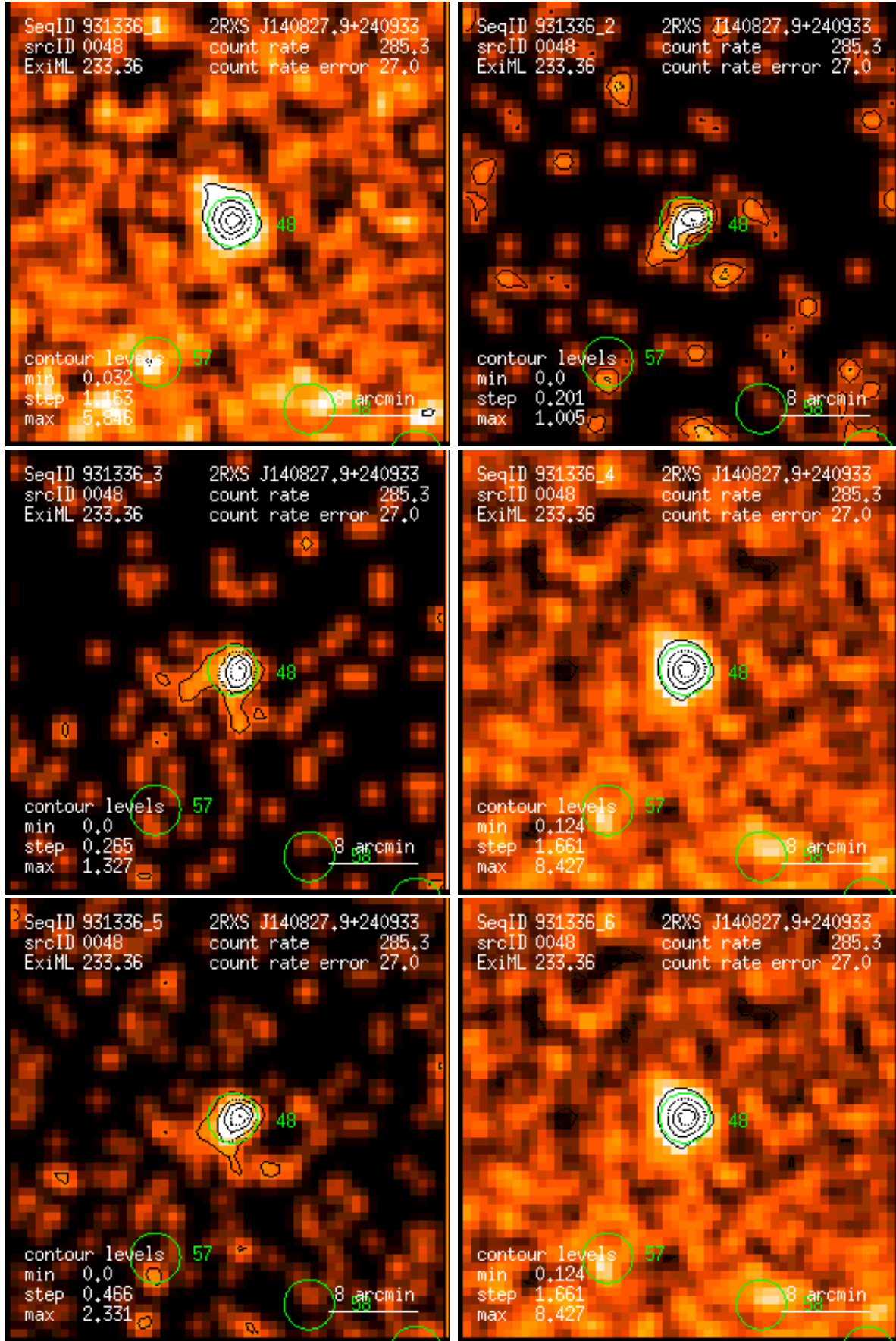
Figure 48: RASS 931336: detection 0048: band rate images, Gaussian filter: (1) PSPC channels 11 – 41, (2) 52 – 90, (3) 91 – 201, (4) 11 – 235, (5) 52 – 201, (6) 11 – 201. Broad band rates in counts/ks. Band rate contour levels in counts/ks/arcmin 2 .
