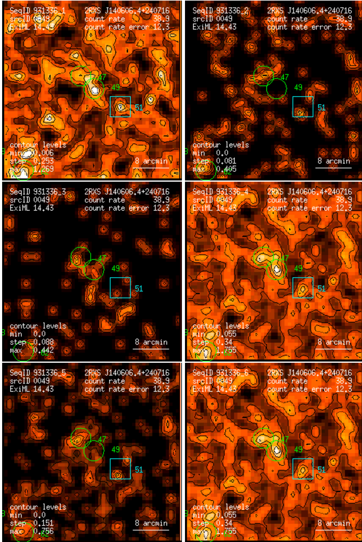
Figure 49: RASS 931336: detection 0049: band rate images, Gaussian filter: (1) PSPC channels 11 – 41, (2) 52 – 90, (3) 91 – 201, (4) 11 – 235, (5) 52 – 201, (6) 11 – 201. Broad band rates in counts/ks. Band rate contour levels in counts/ks/arcmin 2 .
