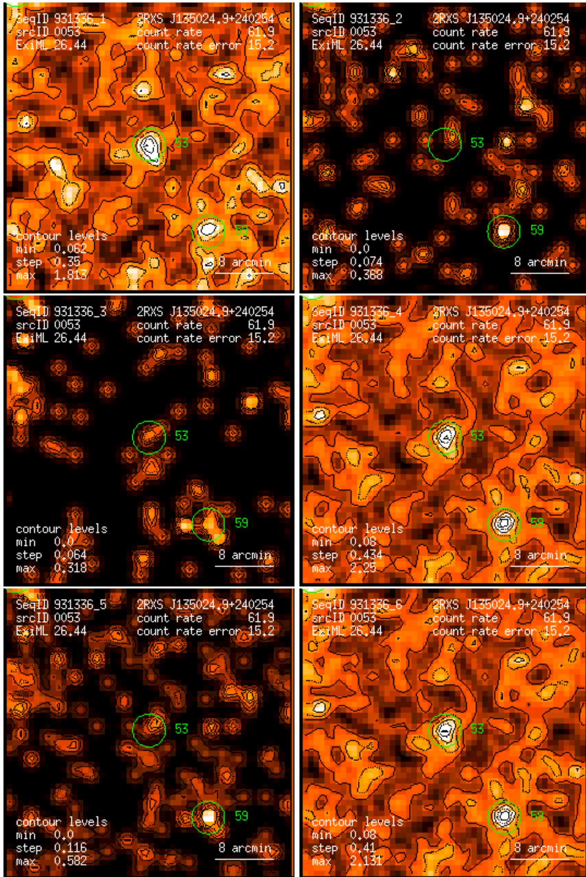
Figure 53: RASS 931336: detection 0053: band rate images, Gaussian filter: (1) PSPC channels 11 – 41, (2) 52 – 90, (3) 91 – 201, (4) 11 – 235, (5) 52 – 201, (6) 11 – 201. Broad band rates in counts/ks. Band rate contour levels in counts/ks/arcmin 2 .
