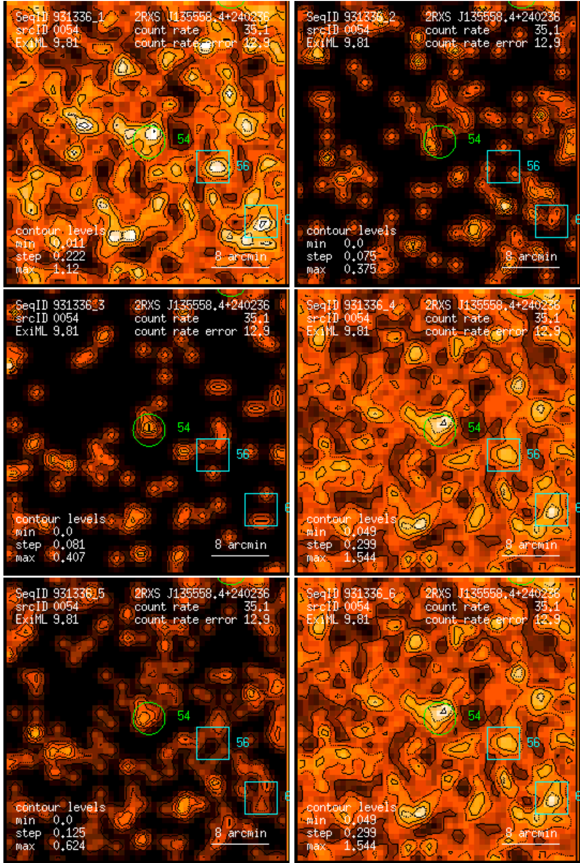
Figure 54: RASS 931336: detection 0054: band rate images, Gaussian filter: (1) PSPC channels 11 – 41, (2) 52 – 90, (3) 91 – 201, (4) 11 – 235, (5) 52 – 201, (6) 11 – 201. Broad band rates in counts/ks. Band rate contour levels in counts/ks/arcmin 2 .
