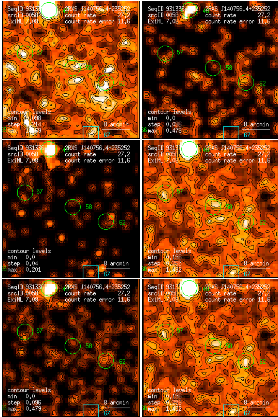
Figure 58: RASS 931336: detection 0058: band rate images, Gaussian filter: (1) PSPC channels 11 – 41, (2) 52 – 90, (3) 91 – 201, (4) 11 – 235, (5) 52 – 201, (6) 11 – 201. Broad band rates in counts/ks. Band rate contour levels in counts/ks/arcmin 2 .
