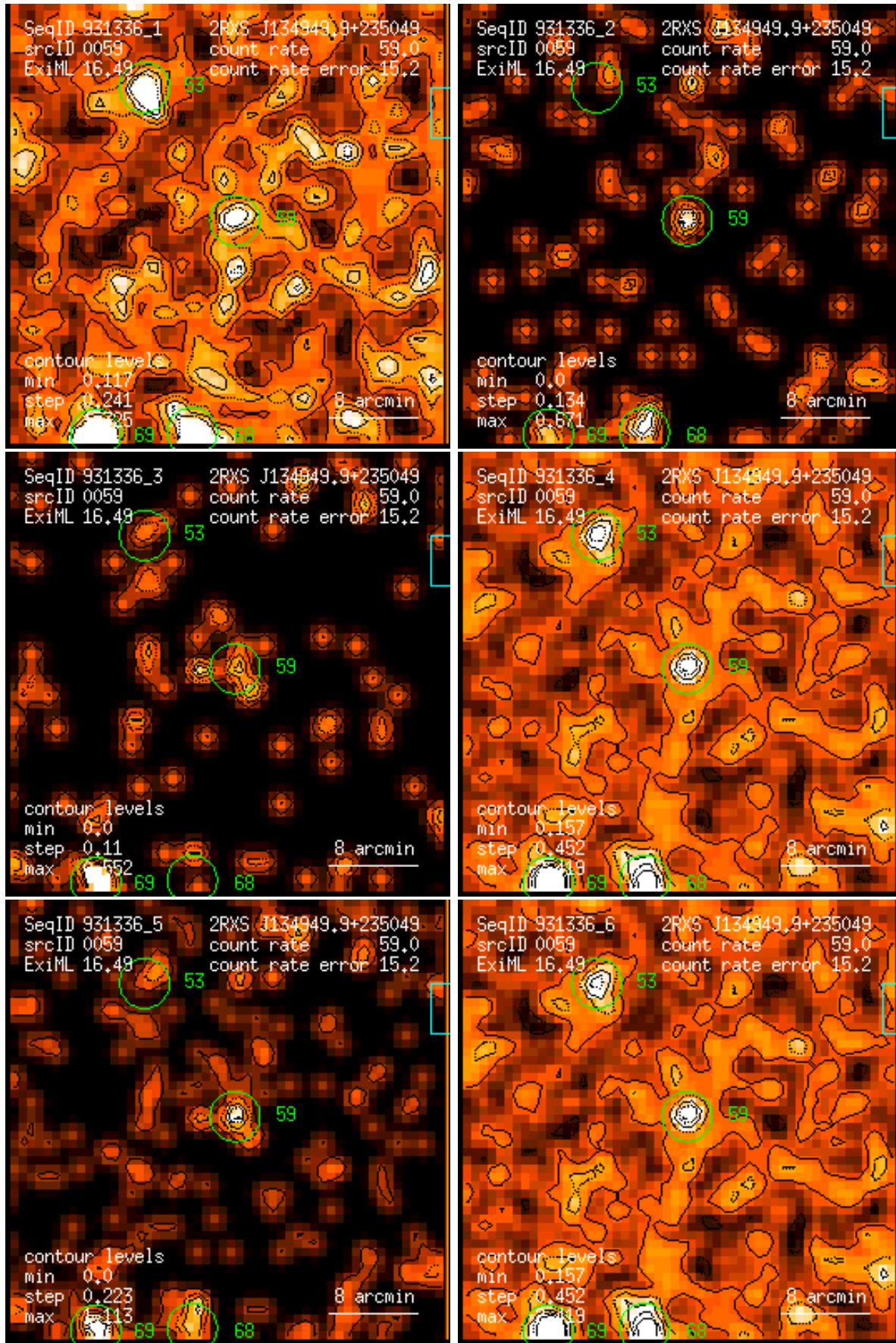
Figure 59: RASS 931336: detection 0059: band rate images, Gaussian filter: (1) PSPC channels 11 – 41, (2) 52 – 90, (3) 91 – 201, (4) 11 – 235, (5) 52 – 201, (6) 11 – 201. Broad band rates in counts/ks. Band rate contour levels in counts/ks/arcmin 2 .
