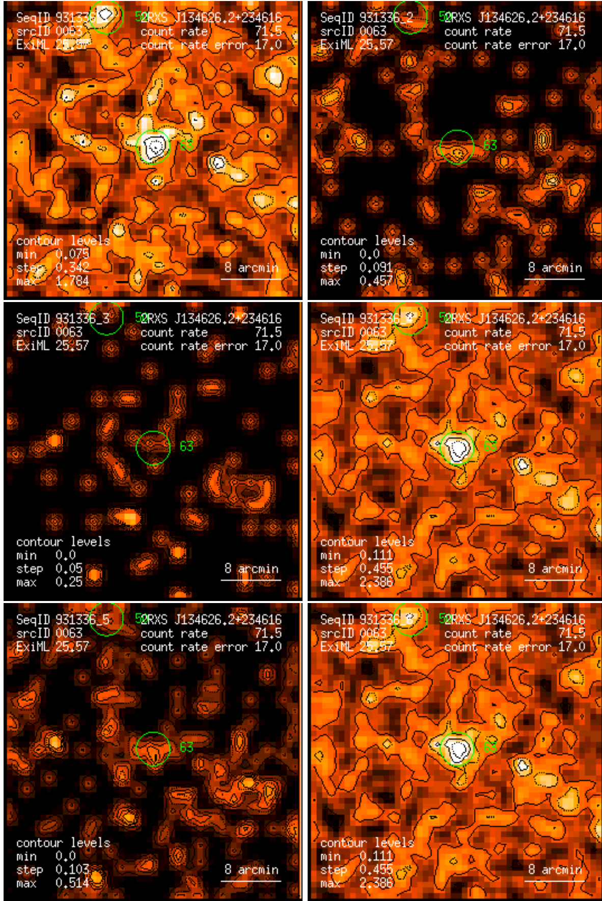
Figure 63: RASS 931336: detection 0063: band rate images, Gaussian filter: (1) PSPC channels 11 – 41, (2) 52 – 90, (3) 91 – 201, (4) 11 – 235, (5) 52 – 201, (6) 11 – 201. Broad band rates in counts/ks. Band rate contour levels in counts/ks/arcmin 2 .
