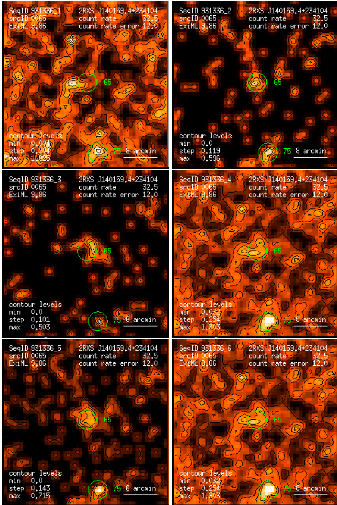
Figure 65: RASS 931336: detection 0065: band rate images, Gaussian filter: (1) PSPC channels 11 – 41, (2) 52 – 90, (3) 91 – 201, (4) 11 – 235, (5) 52 – 201, (6) 11 – 201. Broad band rates in counts/ks. Band rate contour levels in counts/ks/arcmin 2 .
