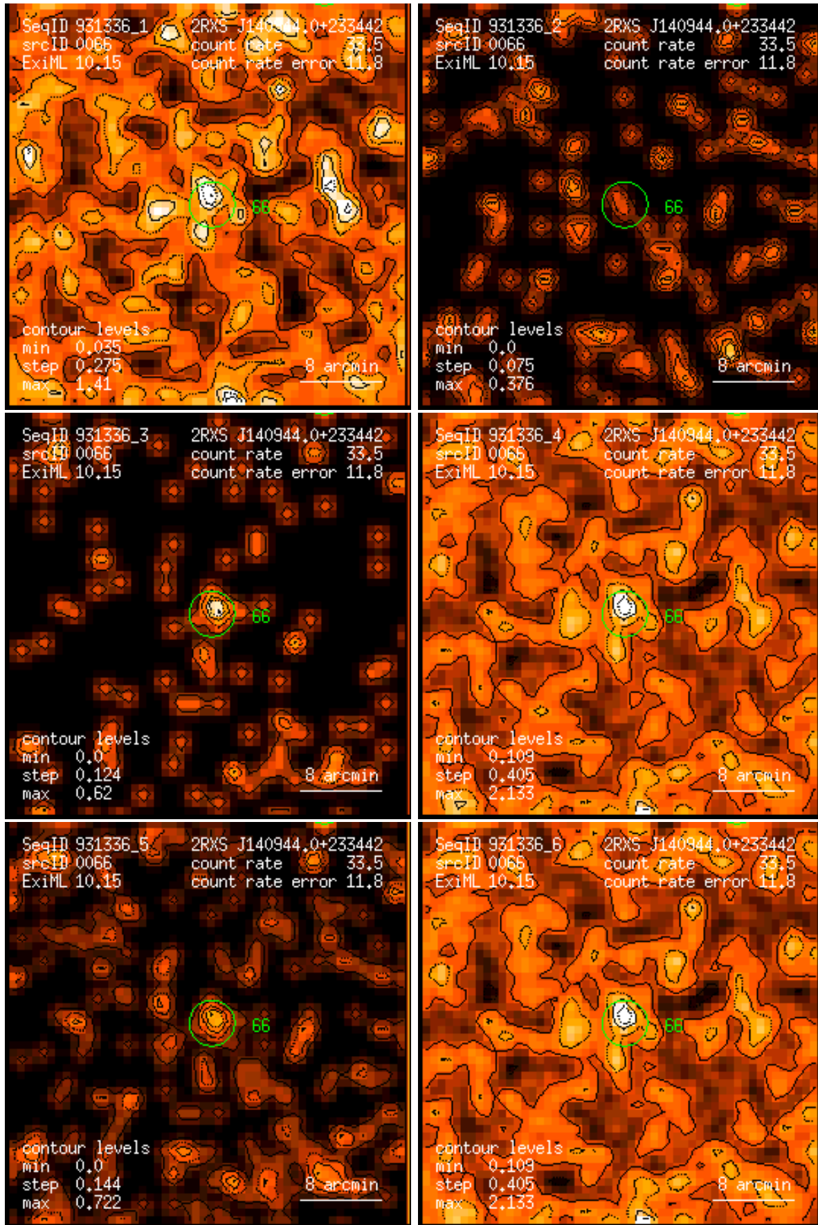
Figure 66: RASS 931336: detection 0066: band rate images, Gaussian filter: (1) PSPC channels 11 – 41, (2) 52 – 90, (3) 91 – 201, (4) 11 – 235, (5) 52 – 201, (6) 11 – 201. Broad band rates in counts/ks. Band rate contour levels in counts/ks/arcmin 2 .
