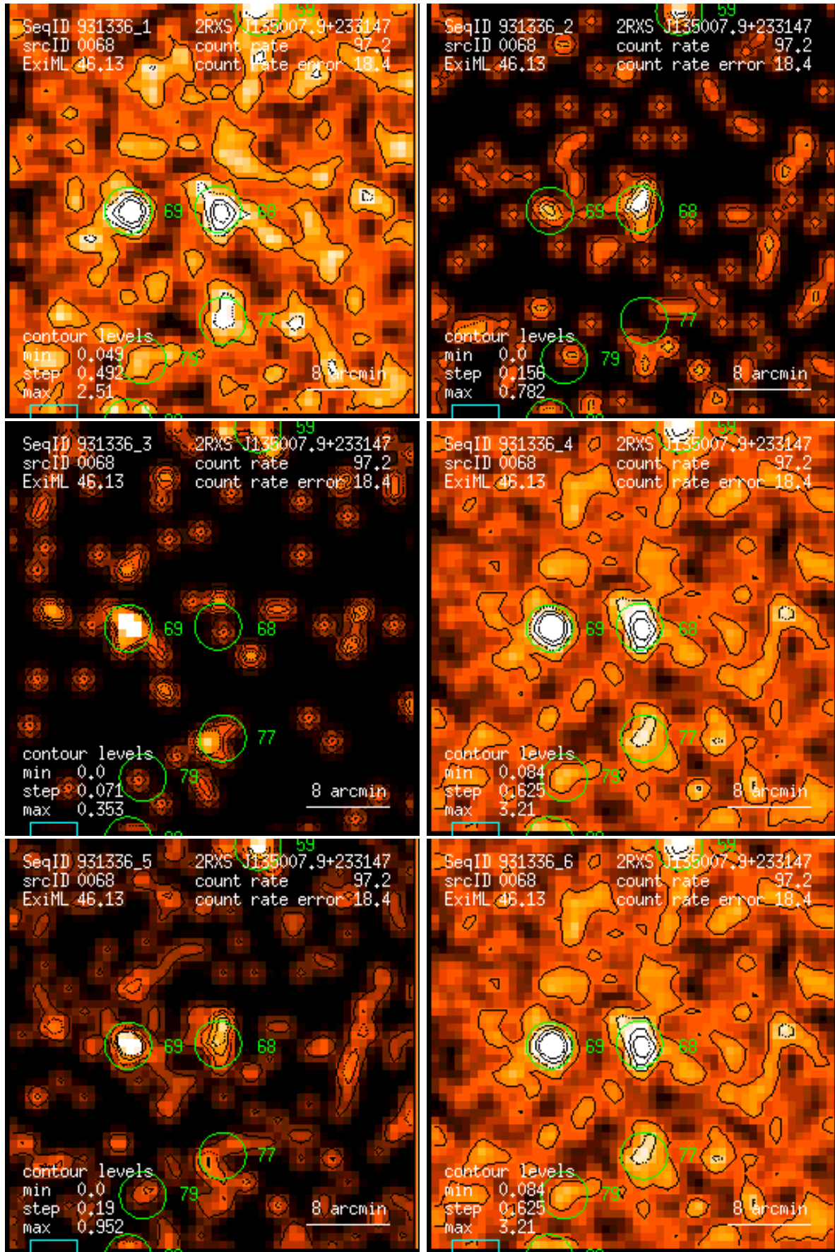
Figure 68: RASS 931336: detection 0068: band rate images, Gaussian filter: (1) PSPC channels 11 – 41, (2) 52 – 90, (3) 91 – 201, (4) 11 – 235, (5) 52 – 201, (6) 11 – 201. Broad band rates in counts/ks. Band rate contour levels in counts/ks/arcmin 2 .
