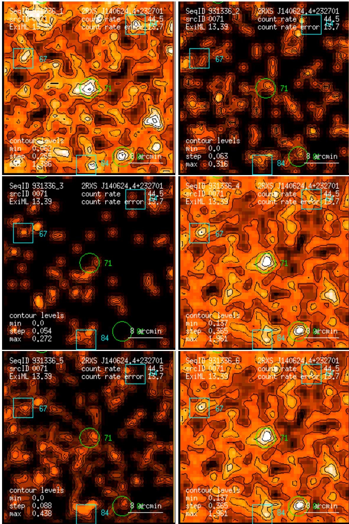
Figure 71: RASS 931336: detection 0071: band rate images, Gaussian filter: (1) PSPC channels 11 – 41, (2) 52 – 90, (3) 91 – 201, (4) 11 – 235, (5) 52 – 201, (6) 11 – 201. Broad band rates in counts/ks. Band rate contour levels in counts/ks/arcmin 2 .
