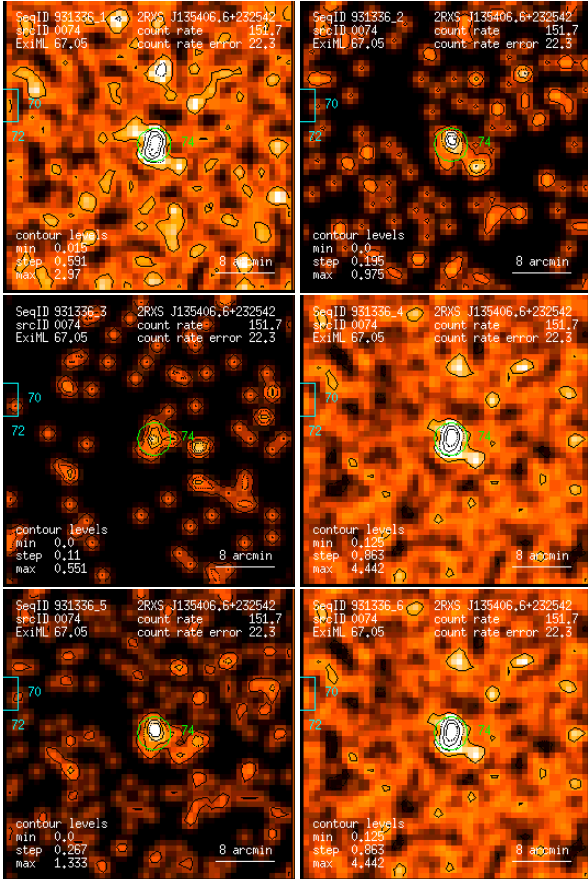
Figure 74: RASS 931336: detection 0074: band rate images, Gaussian filter: (1) PSPC channels 11 – 41, (2) 52 – 90, (3) 91 – 201, (4) 11 – 235, (5) 52 – 201, (6) 11 – 201. Broad band rates in counts/ks. Band rate contour levels in counts/ks/arcmin 2 .
