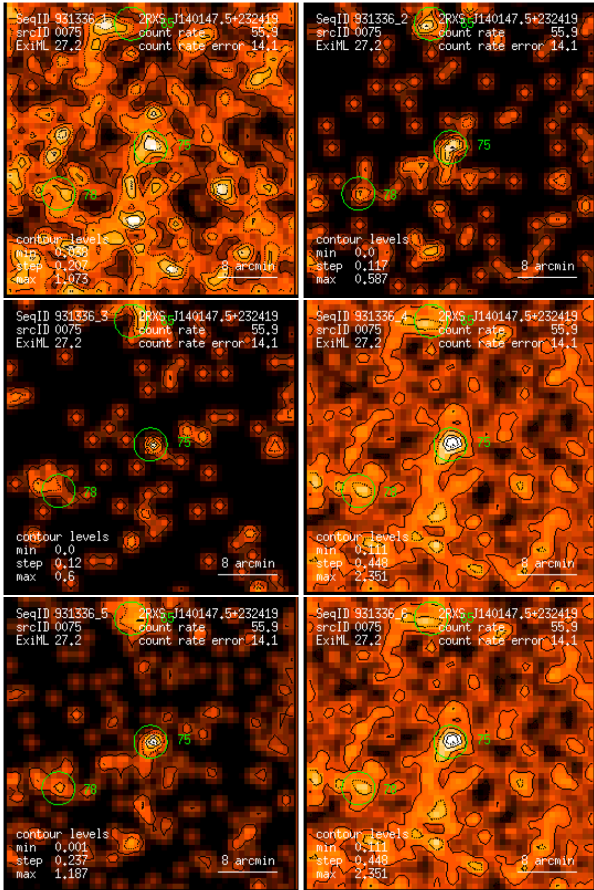
Figure 75: RASS 931336: detection 0075: band rate images, Gaussian filter: (1) PSPC channels 11 – 41, (2) 52 – 90, (3) 91 – 201, (4) 11 – 235, (5) 52 – 201, (6) 11 – 201. Broad band rates in counts/ks. Band rate contour levels in counts/ks/arcmin 2 .
